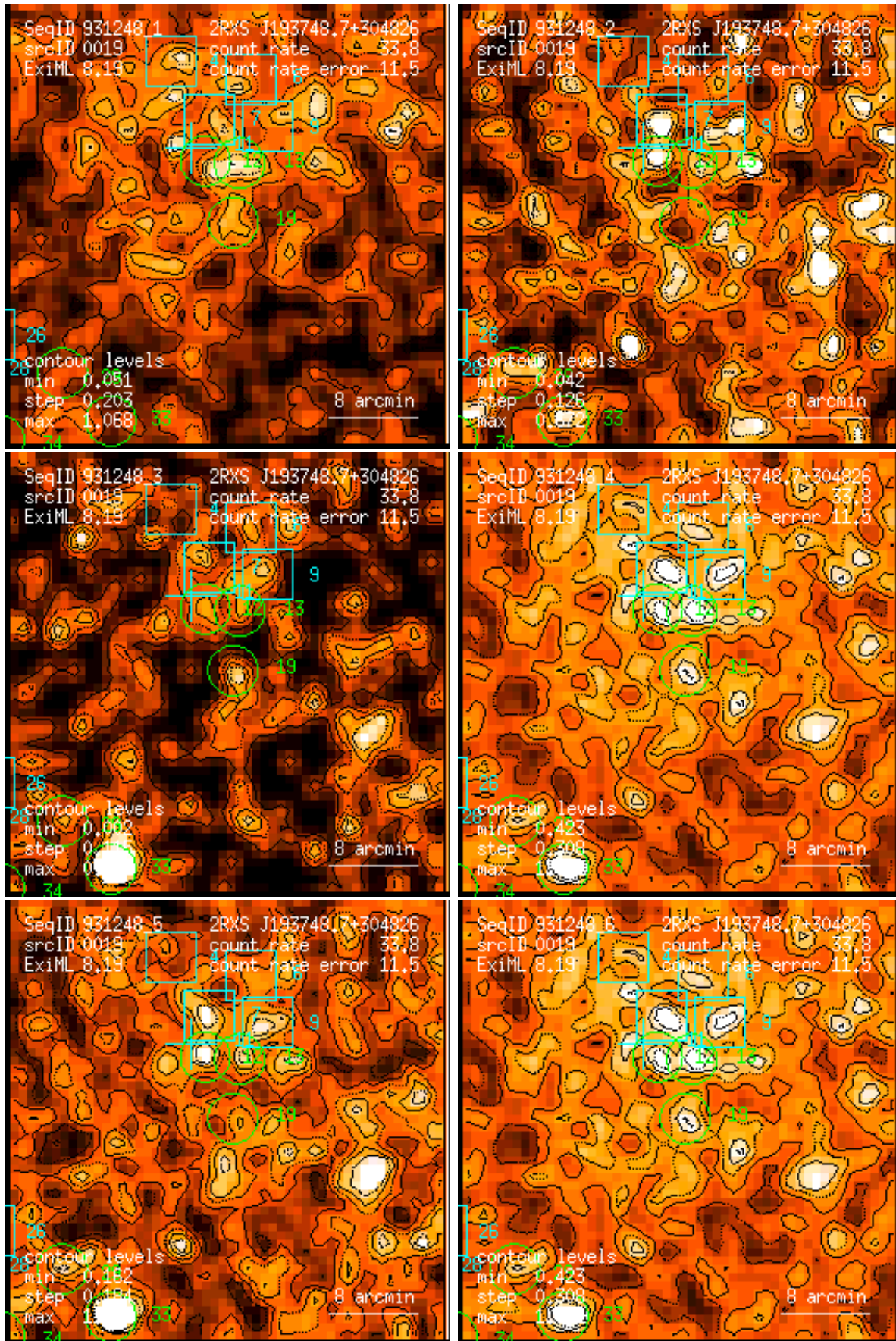
Figure 19: RASS 931248: detection 0019: band rate images, Gaussian filter: (1) PSPC channels 11 – 41, (2) 52 – 90, (3) 91 – 201, (4) 11 – 235, (5) 52 – 201, (6) 11 – 201. Broad band rates in counts/ks. Band rate contour levels in counts/ks/arcmin 2 .
