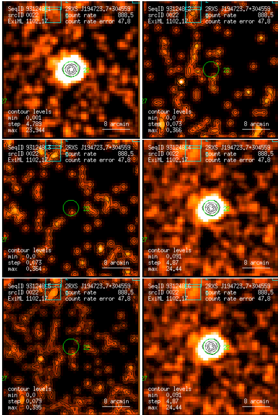
Figure 22: RASS 931248: detection 0022: band rate images, Gaussian filter: (1) PSPC channels 11 – 41, (2) 52 – 90, (3) 91 – 201, (4) 11 – 235, (5) 52 – 201, (6) 11 – 201. Broad band rates in counts/ks. Band rate contour levels in counts/ks/arcmin 2 .
