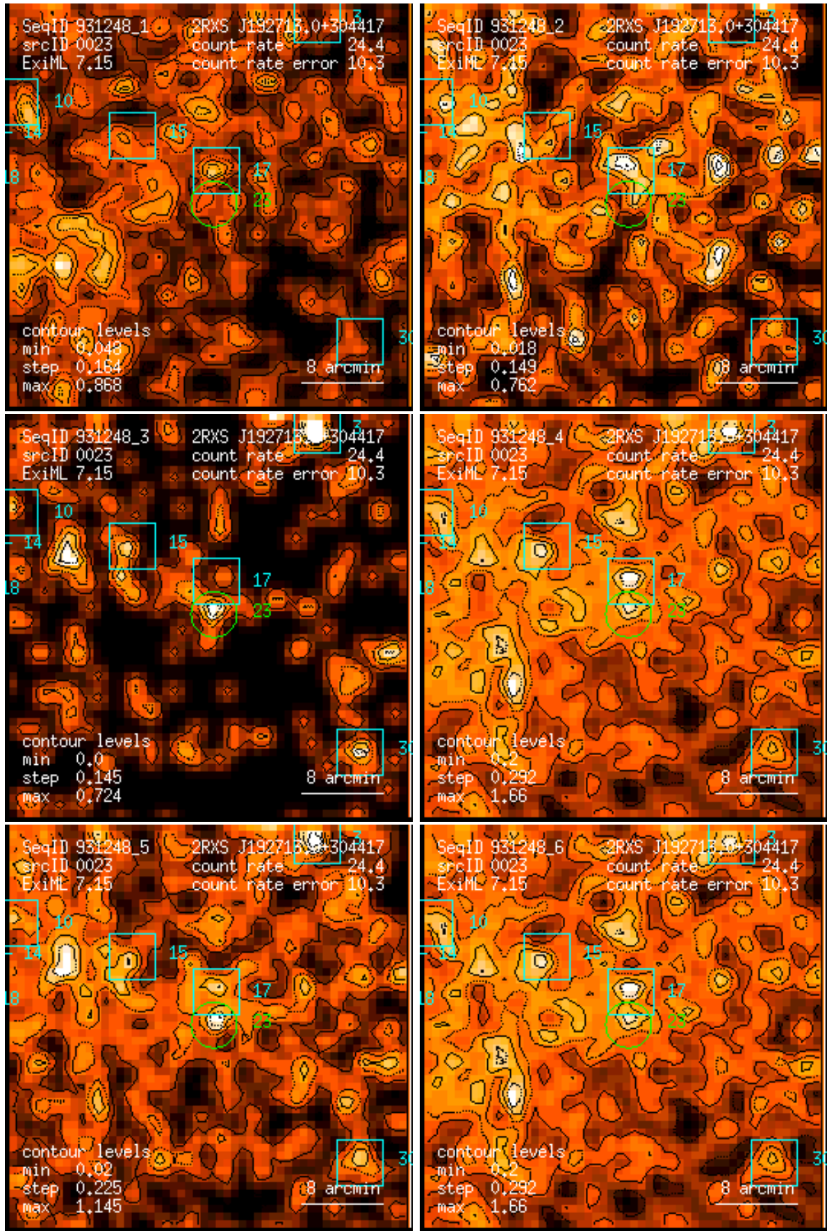
Figure 23: RASS 931248: detection 0023: band rate images, Gaussian filter: (1) PSPC channels 11 – 41, (2) 52 – 90, (3) 91 – 201, (4) 11 – 235, (5) 52 – 201, (6) 11 – 201. Broad band rates in counts/ks. Band rate contour levels in counts/ks/arcmin 2 .
