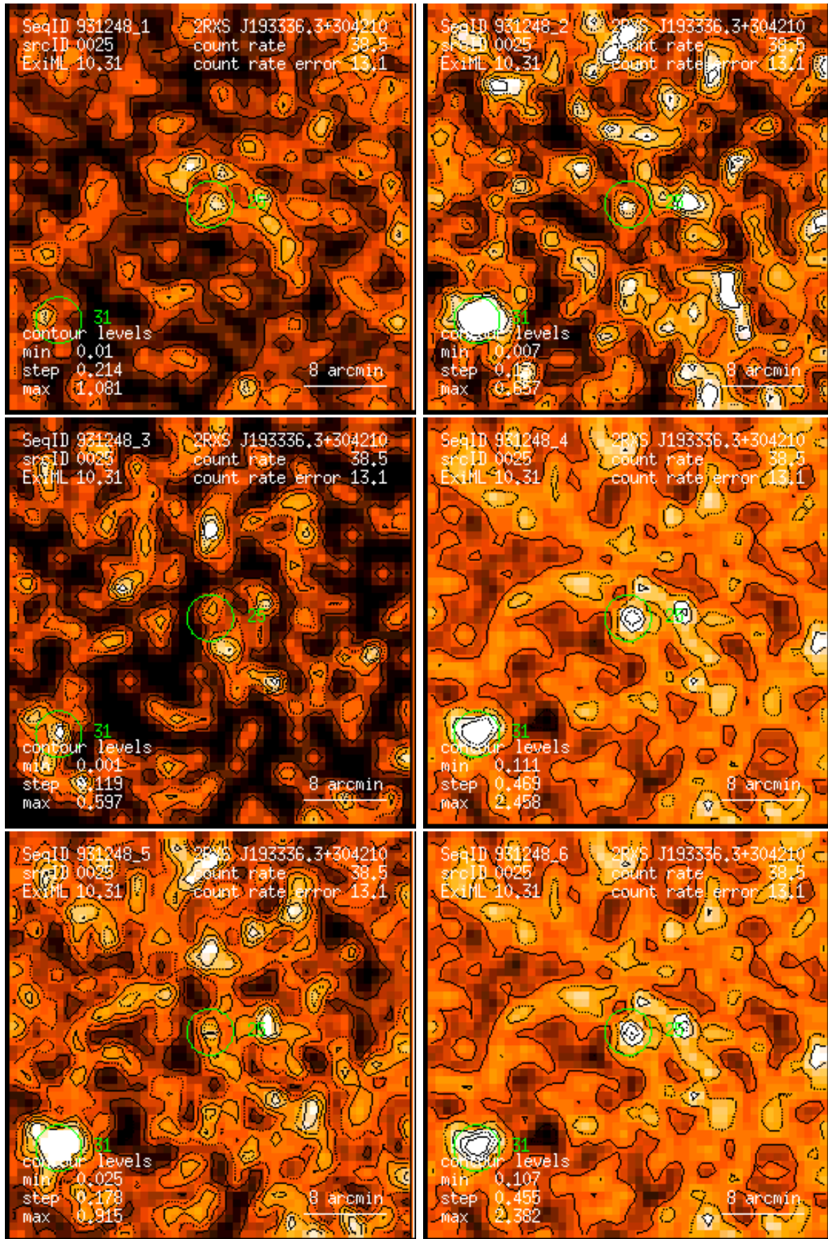
Figure 25: RASS 931248: detection 0025: band rate images, Gaussian filter: (1) PSPC channels 11 – 41, (2) 52 – 90, (3) 91 – 201, (4) 11 – 235, (5) 52 – 201, (6) 11 – 201. Broad band rates in counts/ks. Band rate contour levels in counts/ks/arcmin 2 .
