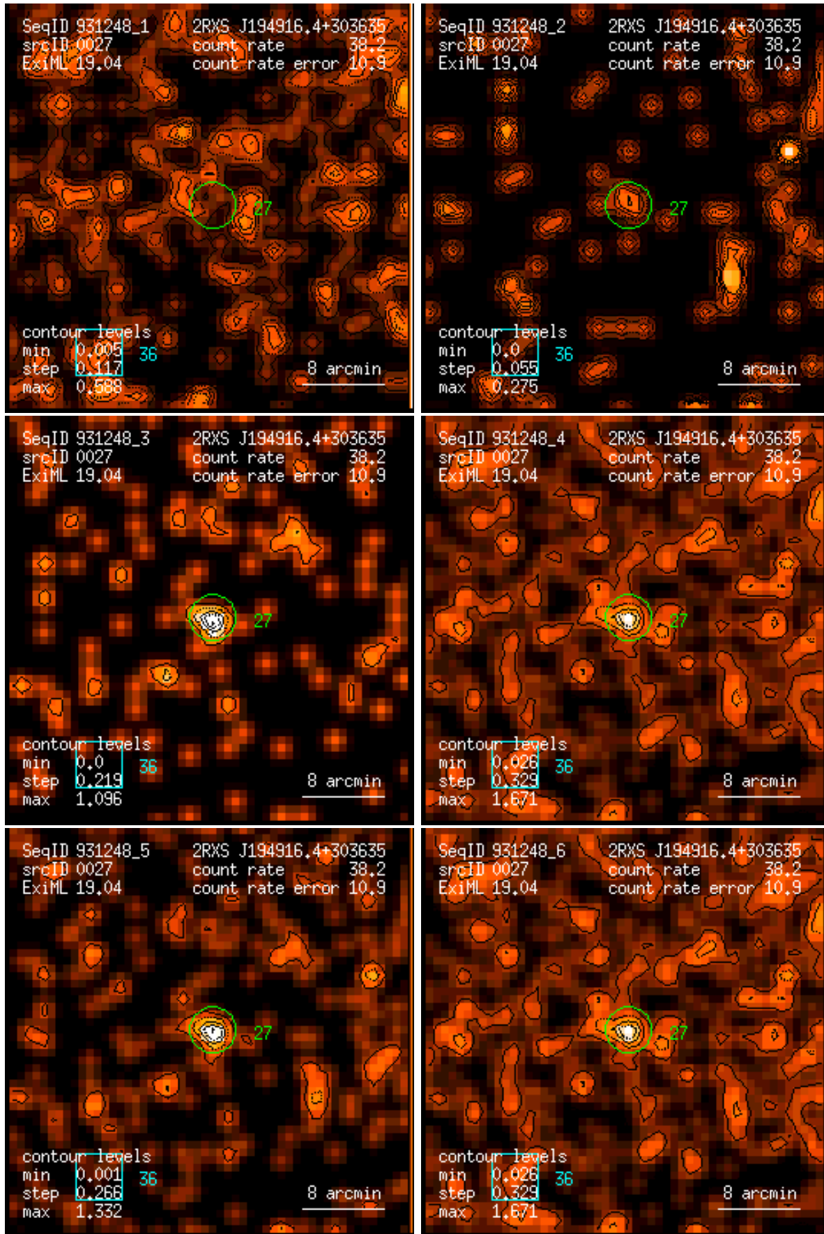
Figure 27: RASS 931248: detection 0027: band rate images, Gaussian filter: (1) PSPC channels 11 – 41, (2) 52 – 90, (3) 91 – 201, (4) 11 – 235, (5) 52 – 201, (6) 11 – 201. Broad band rates in counts/ks. Band rate contour levels in counts/ks/arcmin 2 .
