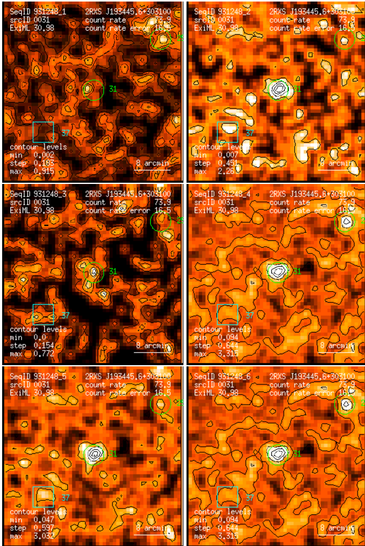
Figure 31: RASS 931248: detection 0031: band rate images, Gaussian filter: (1) PSPC channels 11 – 41, (2) 52 – 90, (3) 91 – 201, (4) 11 – 235, (5) 52 – 201, (6) 11 – 201. Broad band rates in counts/ks. Band rate contour levels in counts/ks/arcmin 2 .
