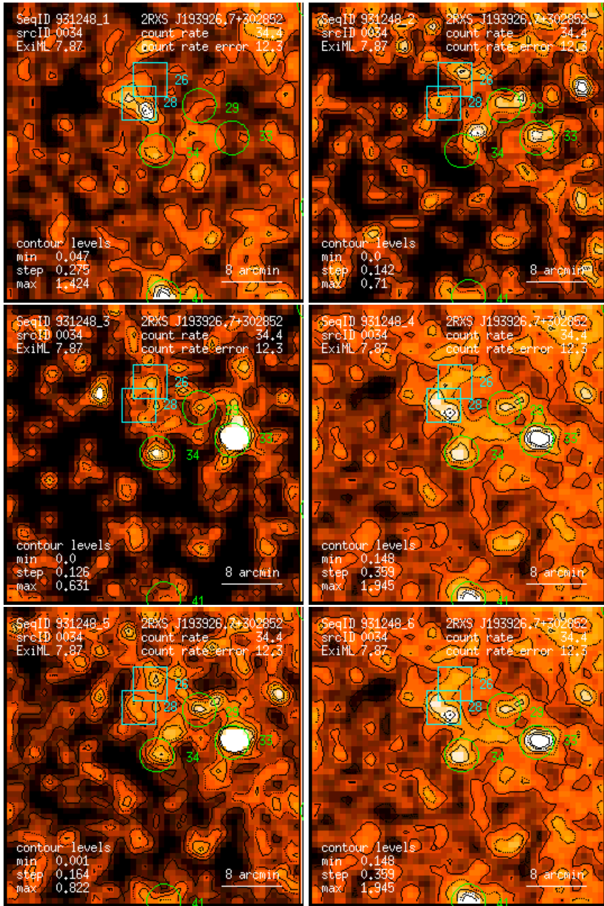
Figure 34: RASS 931248: detection 0034: band rate images, Gaussian filter: (1) PSPC channels 11 – 41, (2) 52 – 90, (3) 91 – 201, (4) 11 – 235, (5) 52 – 201, (6) 11 – 201. Broad band rates in counts/ks. Band rate contour levels in counts/ks/arcmin 2 .
