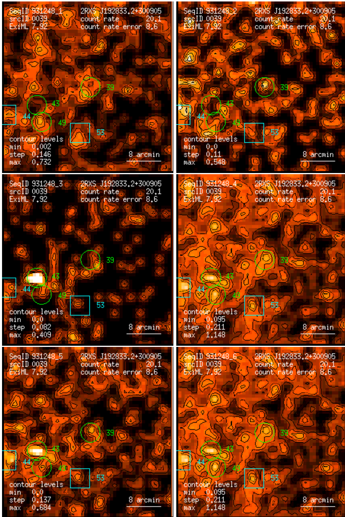
Figure 39: RASS 931248: detection 0039: band rate images, Gaussian filter: (1) PSPC channels 11 – 41, (2) 52 – 90, (3) 91 – 201, (4) 11 – 235, (5) 52 – 201, (6) 11 – 201. Broad band rates in counts/ks. Band rate contour levels in counts/ks/arcmin 2 .
