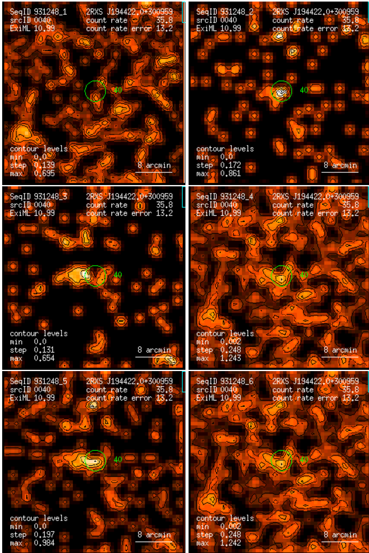
Figure 40: RASS 931248: detection 0040: band rate images, Gaussian filter: (1) PSPC channels 11 – 41, (2) 52 – 90, (3) 91 – 201, (4) 11 – 235, (5) 52 – 201, (6) 11 – 201. Broad band rates in counts/ks. Band rate contour levels in counts/ks/arcmin 2 .
