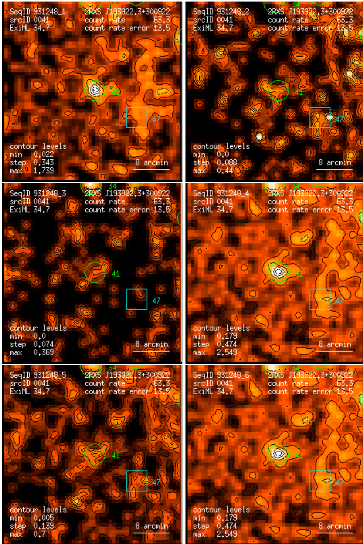
Figure 41: RASS 931248: detection 0041: band rate images, Gaussian filter: (1) PSPC channels 11 – 41, (2) 52 – 90, (3) 91 – 201, (4) 11 – 235, (5) 52 – 201, (6) 11 – 201. Broad band rates in counts/ks. Band rate contour levels in counts/ks/arcmin 2 .
