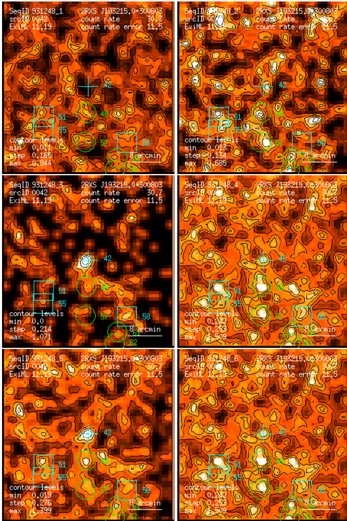
Figure 42: RASS 931248: detection 0042: band rate images, Gaussian filter: (1) PSPC channels 11 – 41, (2) 52 – 90, (3) 91 – 201, (4) 11 – 235, (5) 52 – 201, (6) 11 – 201. Broad band rates in counts/ks. Band rate contour levels in counts/ks/arcmin 2 .
