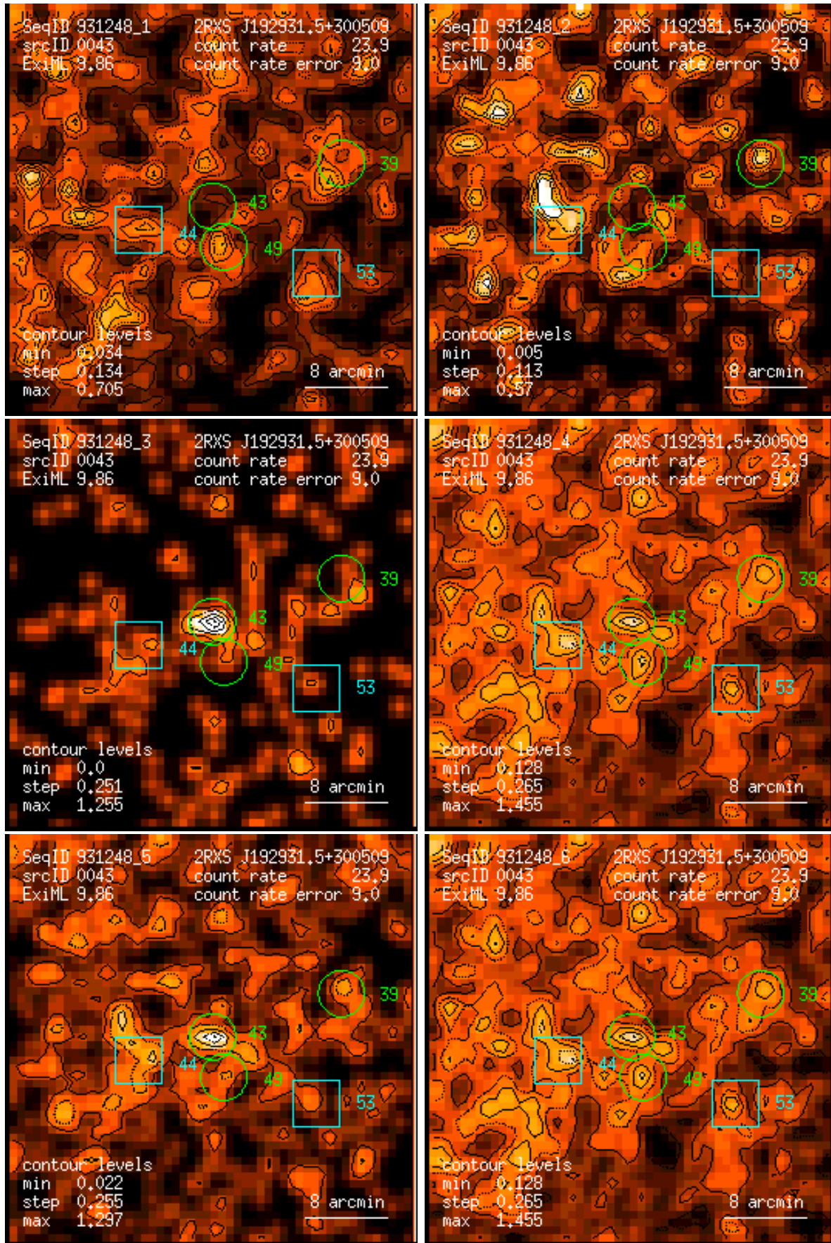
Figure 43: RASS 931248: detection 0043: band rate images, Gaussian filter: (1) PSPC channels 11 – 41, (2) 52 – 90, (3) 91 – 201, (4) 11 – 235, (5) 52 – 201, (6) 11 – 201. Broad band rates in counts/ks. Band rate contour levels in counts/ks/arcmin 2 .
