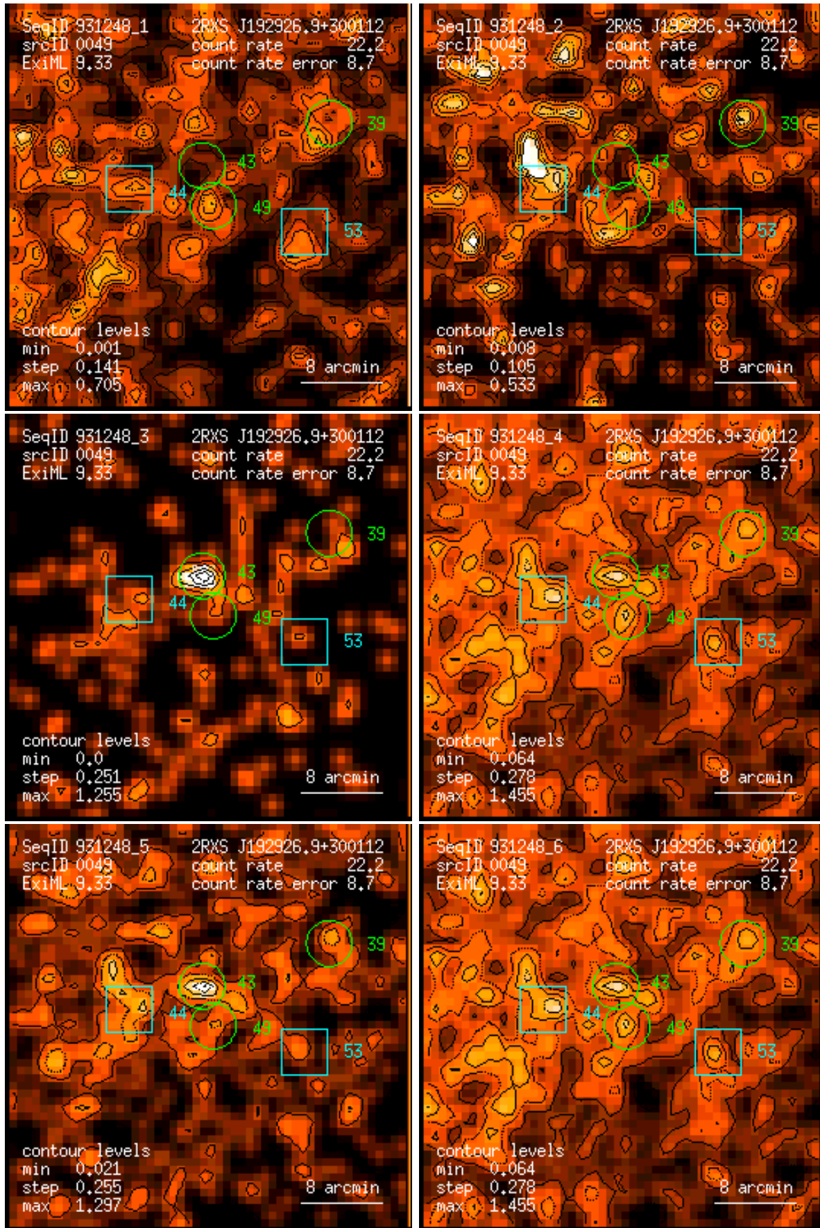
Figure 49: RASS 931248: detection 0049: band rate images, Gaussian filter: (1) PSPC channels 11 – 41, (2) 52 – 90, (3) 91 – 201, (4) 11 – 235, (5) 52 – 201, (6) 11 – 201. Broad band rates in counts/ks. Band rate contour levels in counts/ks/arcmin 2 .
