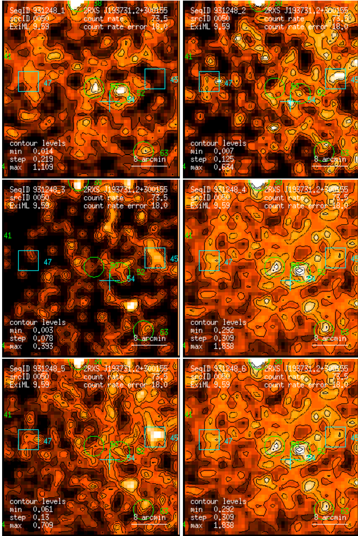
Figure 50: RASS 931248: detection 0050: band rate images, Gaussian filter: (1) PSPC channels 11 – 41, (2) 52 – 90, (3) 91 – 201, (4) 11 – 235, (5) 52 – 201, (6) 11 – 201. Broad band rates in counts/ks. Band rate contour levels in counts/ks/arcmin 2 .
