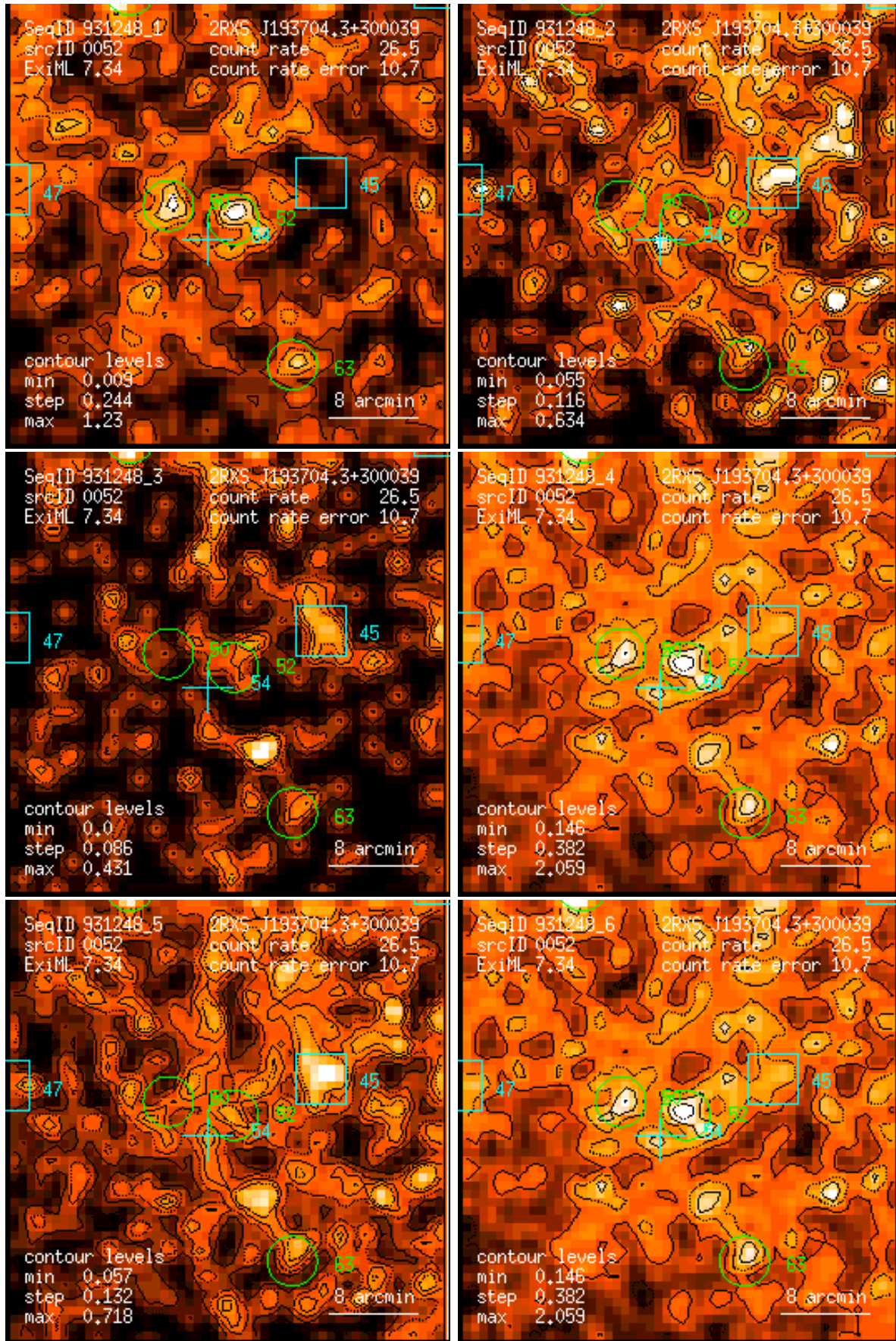
Figure 52: RASS 931248: detection 0052: band rate images, Gaussian filter: (1) PSPC channels 11 – 41, (2) 52 – 90, (3) 91 – 201, (4) 11 – 235, (5) 52 – 201, (6) 11 – 201. Broad band rates in counts/ks. Band rate contour levels in counts/ks/arcmin 2 .
