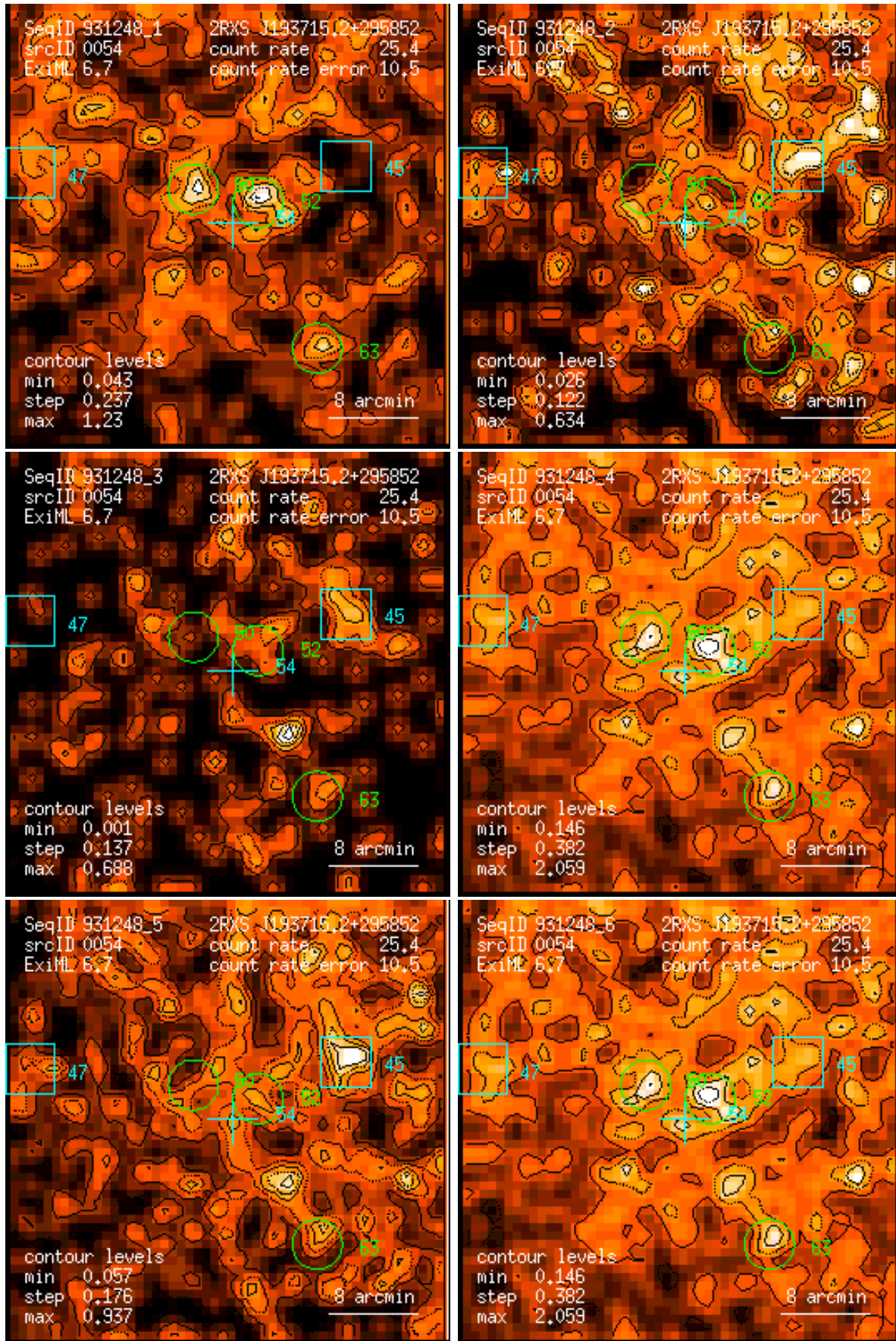
Figure 54: RASS 931248: detection 0054: band rate images, Gaussian filter: (1) PSPC channels 11 – 41, (2) 52 – 90, (3) 91 – 201, (4) 11 – 235, (5) 52 – 201, (6) 11 – 201. Broad band rates in counts/ks. Band rate contour levels in counts/ks/arcmin 2 .
