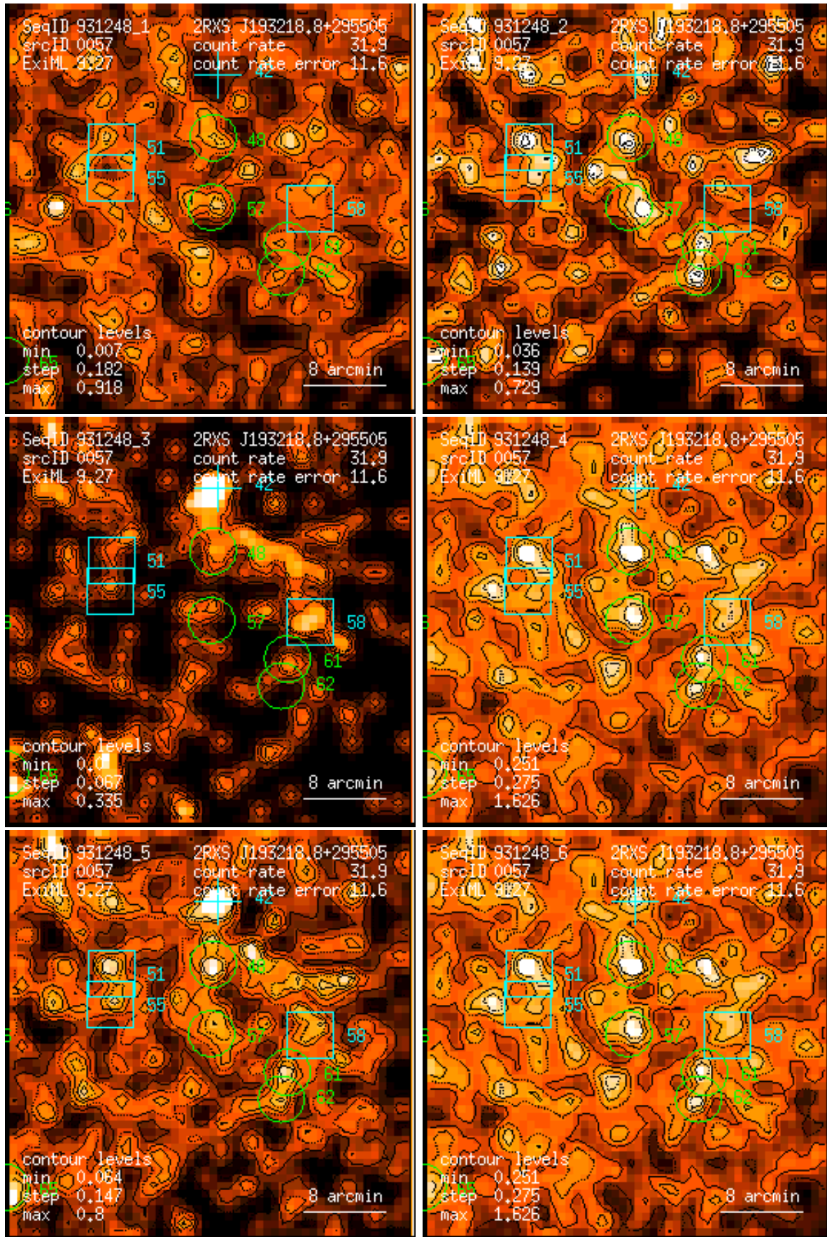
Figure 57: RASS 931248: detection 0057: band rate images, Gaussian filter: (1) PSPC channels 11 – 41, (2) 52 – 90, (3) 91 – 201, (4) 11 – 235, (5) 52 – 201, (6) 11 – 201. Broad band rates in counts/ks. Band rate contour levels in counts/ks/arcmin 2 .
