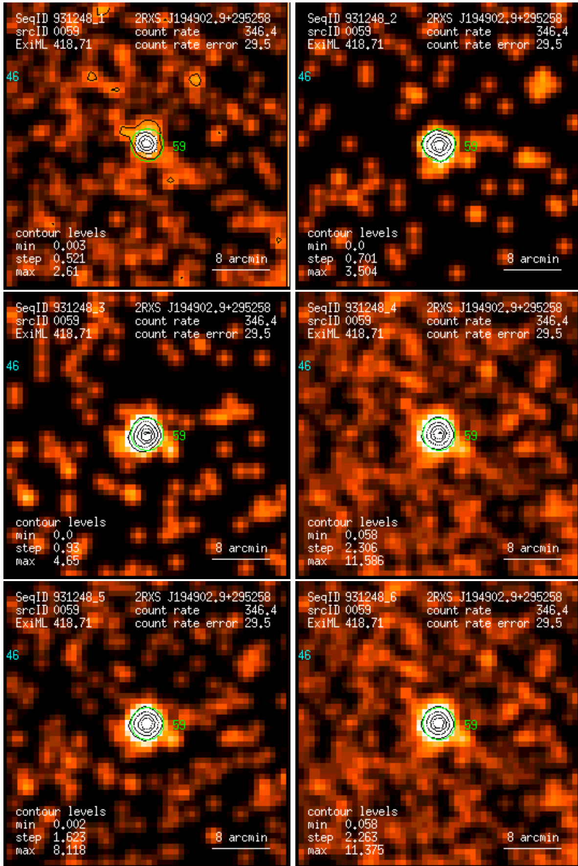
Figure 59: RASS 931248: detection 0059: band rate images, Gaussian filter: (1) PSPC channels 11 – 41, (2) 52 – 90, (3) 91 – 201, (4) 11 – 235, (5) 52 – 201, (6) 11 – 201. Broad band rates in counts/ks. Band rate contour levels in counts/ks/arcmin 2 .
