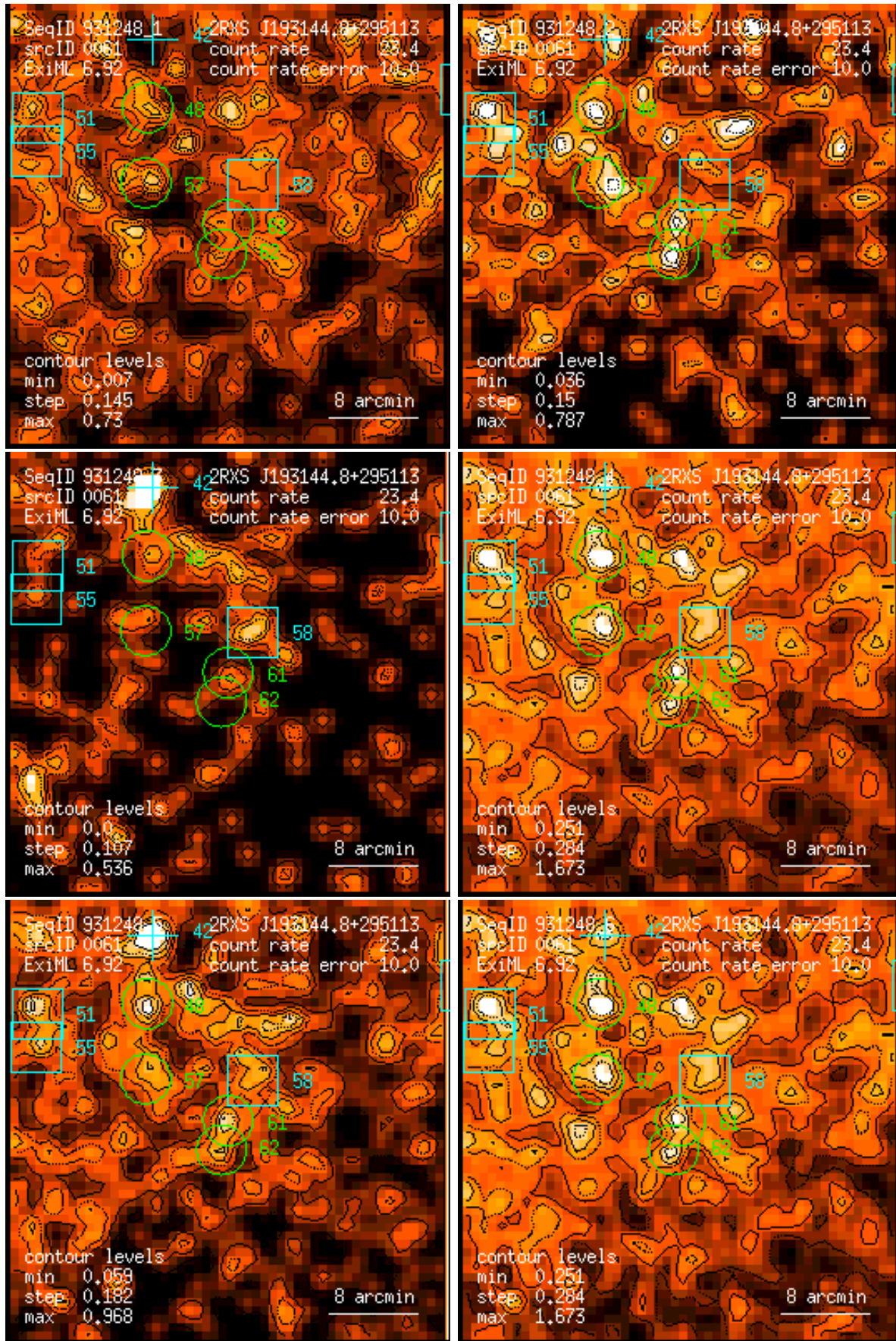
Figure 61: RASS 931248: detection 0061: band rate images, Gaussian filter: (1) PSPC channels 11 – 41, (2) 52 – 90, (3) 91 – 201, (4) 11 – 235, (5) 52 – 201, (6) 11 – 201. Broad band rates in counts/ks. Band rate contour levels in counts/ks/arcmin 2 .
