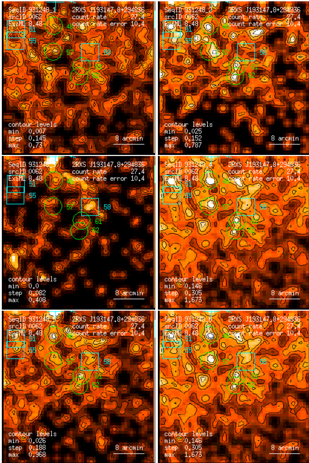
Figure 62: RASS 931248: detection 0062: band rate images, Gaussian filter: (1) PSPC channels 11 – 41, (2) 52 – 90, (3) 91 – 201, (4) 11 – 235, (5) 52 – 201, (6) 11 – 201. Broad band rates in counts/ks. Band rate contour levels in counts/ks/arcmin 2 .
