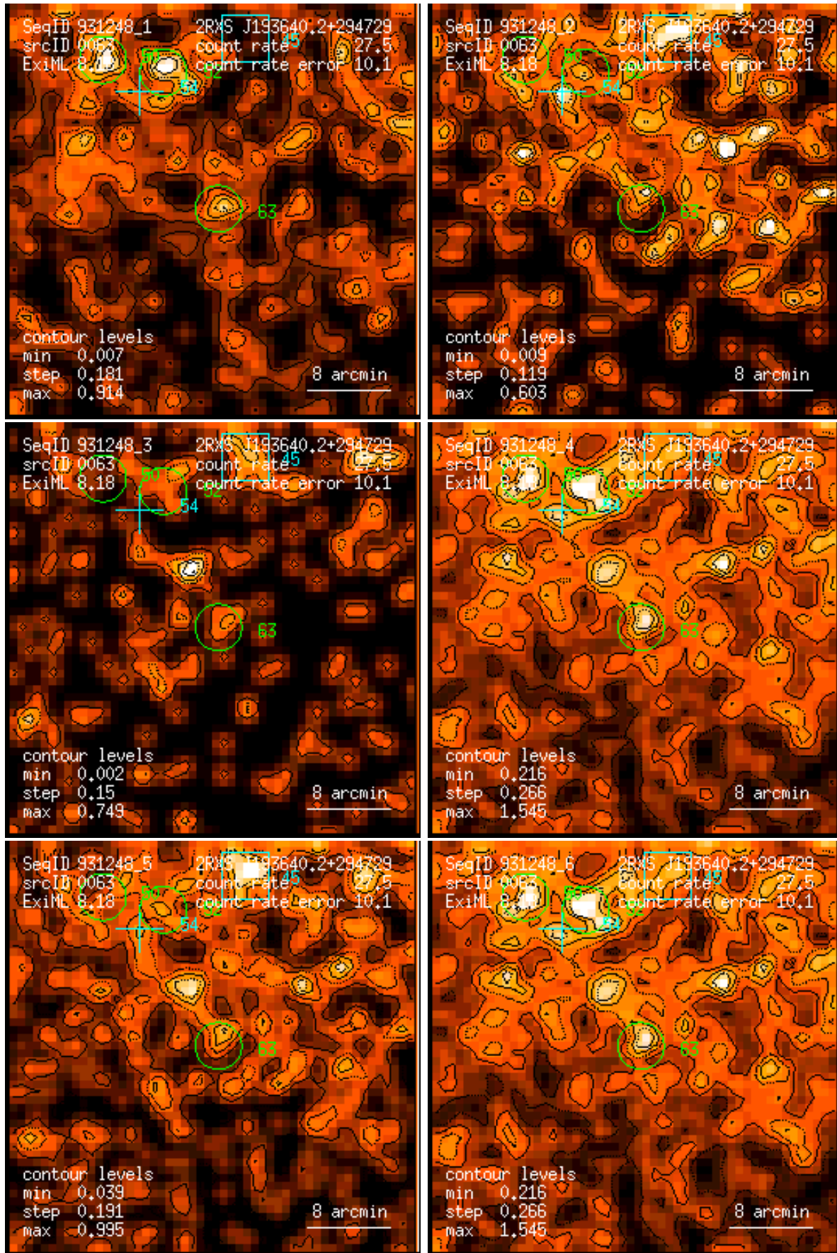
Figure 63: RASS 931248: detection 0063: band rate images, Gaussian filter: (1) PSPC channels 11 – 41, (2) 52 – 90, (3) 91 – 201, (4) 11 – 235, (5) 52 – 201, (6) 11 – 201. Broad band rates in counts/ks. Band rate contour levels in counts/ks/arcmin 2 .
