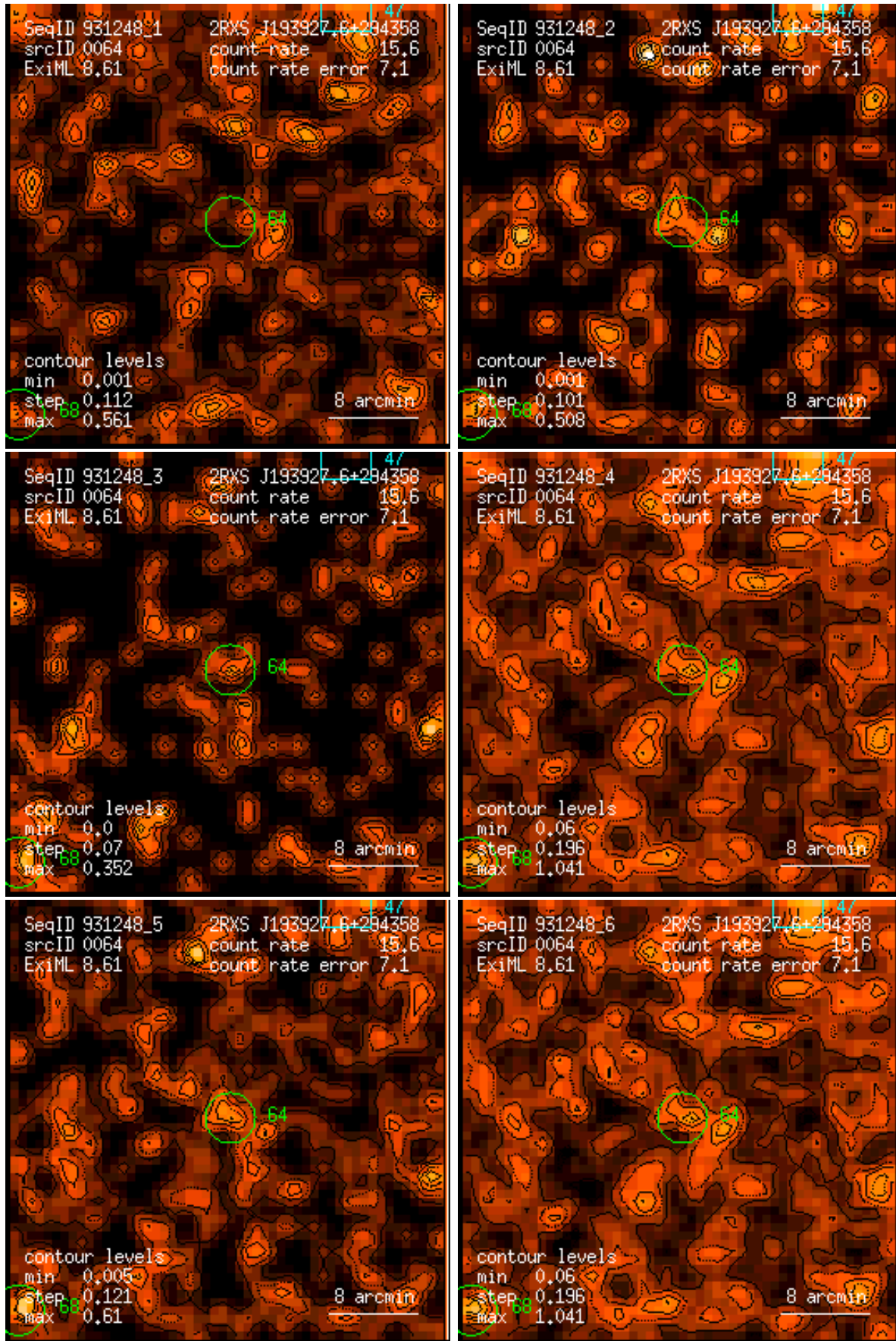
Figure 64: RASS 931248: detection 0064: band rate images, Gaussian filter: (1) PSPC channels 11 – 41, (2) 52 – 90, (3) 91 – 201, (4) 11 – 235, (5) 52 – 201, (6) 11 – 201. Broad band rates in counts/ks. Band rate contour levels in counts/ks/arcmin 2 .
