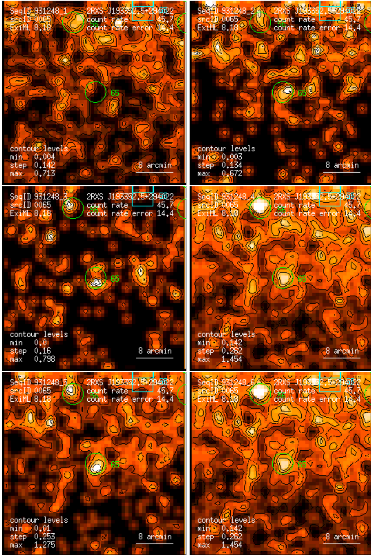
Figure 65: RASS 931248: detection 0065: band rate images, Gaussian filter: (1) PSPC channels 11 – 41, (2) 52 – 90, (3) 91 – 201, (4) 11 – 235, (5) 52 – 201, (6) 11 – 201. Broad band rates in counts/ks. Band rate contour levels in counts/ks/arcmin 2 .
