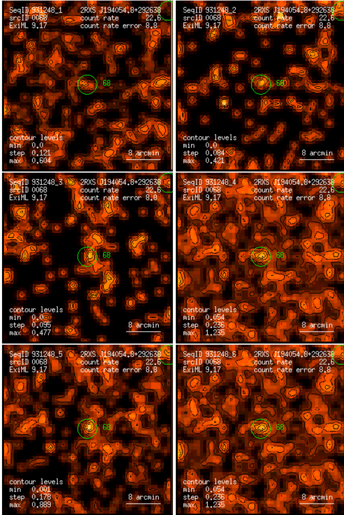
Figure 68: RASS 931248: detection 0068: band rate images, Gaussian filter: (1) PSPC channels 11 – 41, (2) 52 – 90, (3) 91 – 201, (4) 11 – 235, (5) 52 – 201, (6) 11 – 201. Broad band rates in counts/ks. Band rate contour levels in counts/ks/arcmin 2 .
