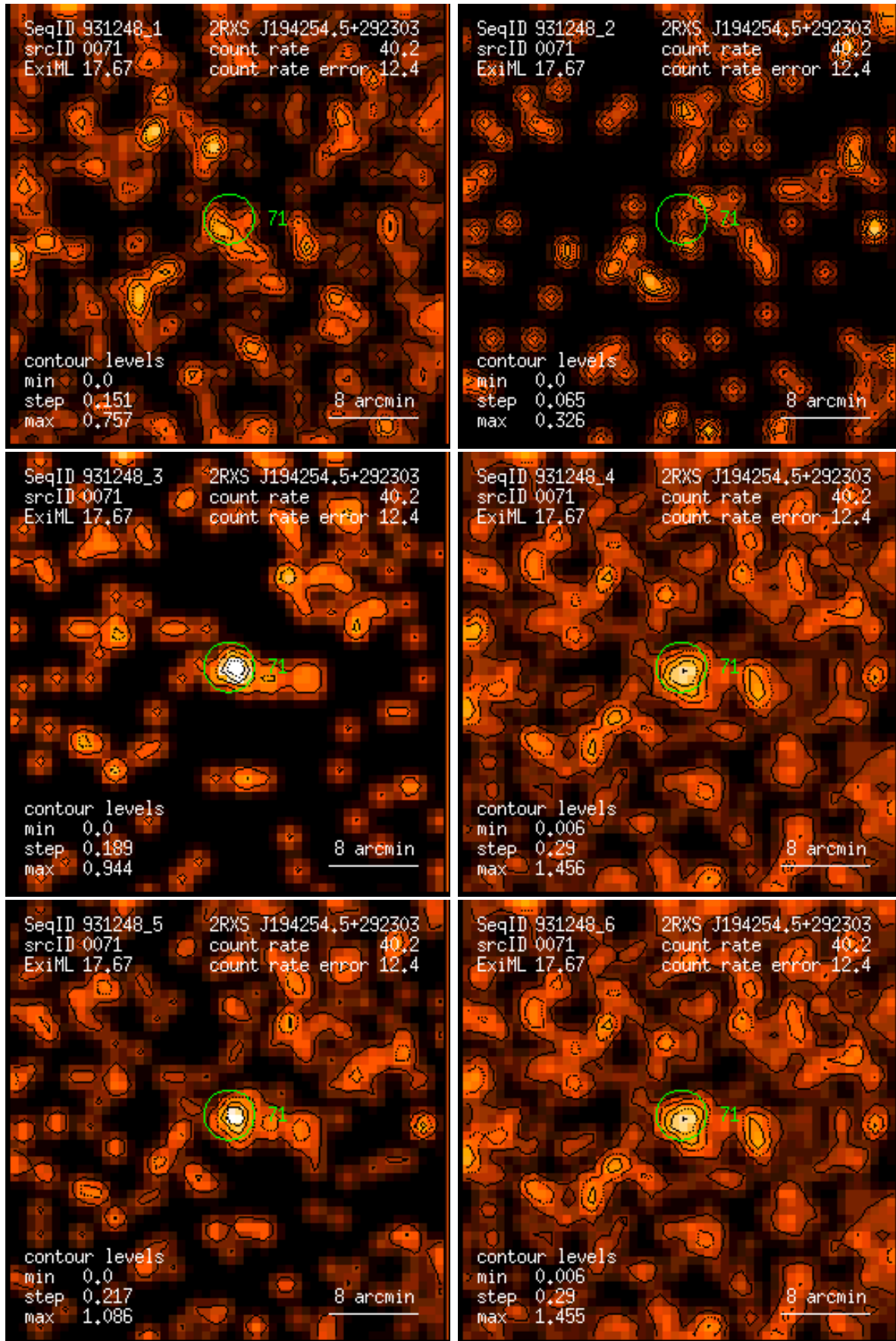
Figure 71: RASS 931248: detection 0071: band rate images, Gaussian filter: (1) PSPC channels 11 – 41, (2) 52 – 90, (3) 91 – 201, (4) 11 – 235, (5) 52 – 201, (6) 11 – 201. Broad band rates in counts/ks. Band rate contour levels in counts/ks/arcmin 2 .
