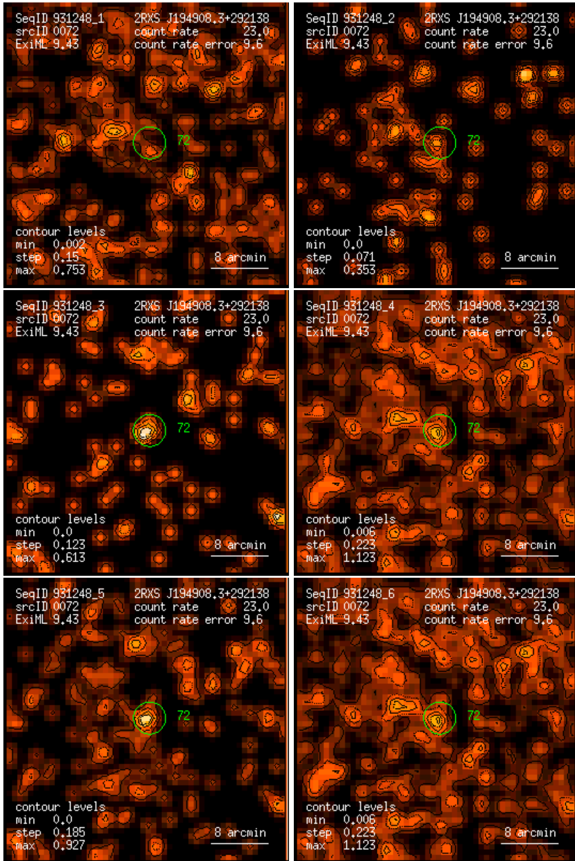
Figure 72: RASS 931248: detection 0072: band rate images, Gaussian filter: (1) PSPC channels 11 – 41, (2) 52 – 90, (3) 91 – 201, (4) 11 – 235, (5) 52 – 201, (6) 11 – 201. Broad band rates in counts/ks. Band rate contour levels in counts/ks/arcmin 2 .
