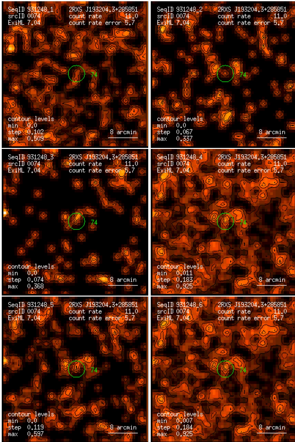
Figure 74: RASS 931248: detection 0074: band rate images, Gaussian filter: (1) PSPC channels 11 – 41, (2) 52 – 90, (3) 91 – 201, (4) 11 – 235, (5) 52 – 201, (6) 11 – 201. Broad band rates in counts/ks. Band rate contour levels in counts/ks/arcmin 2 .
