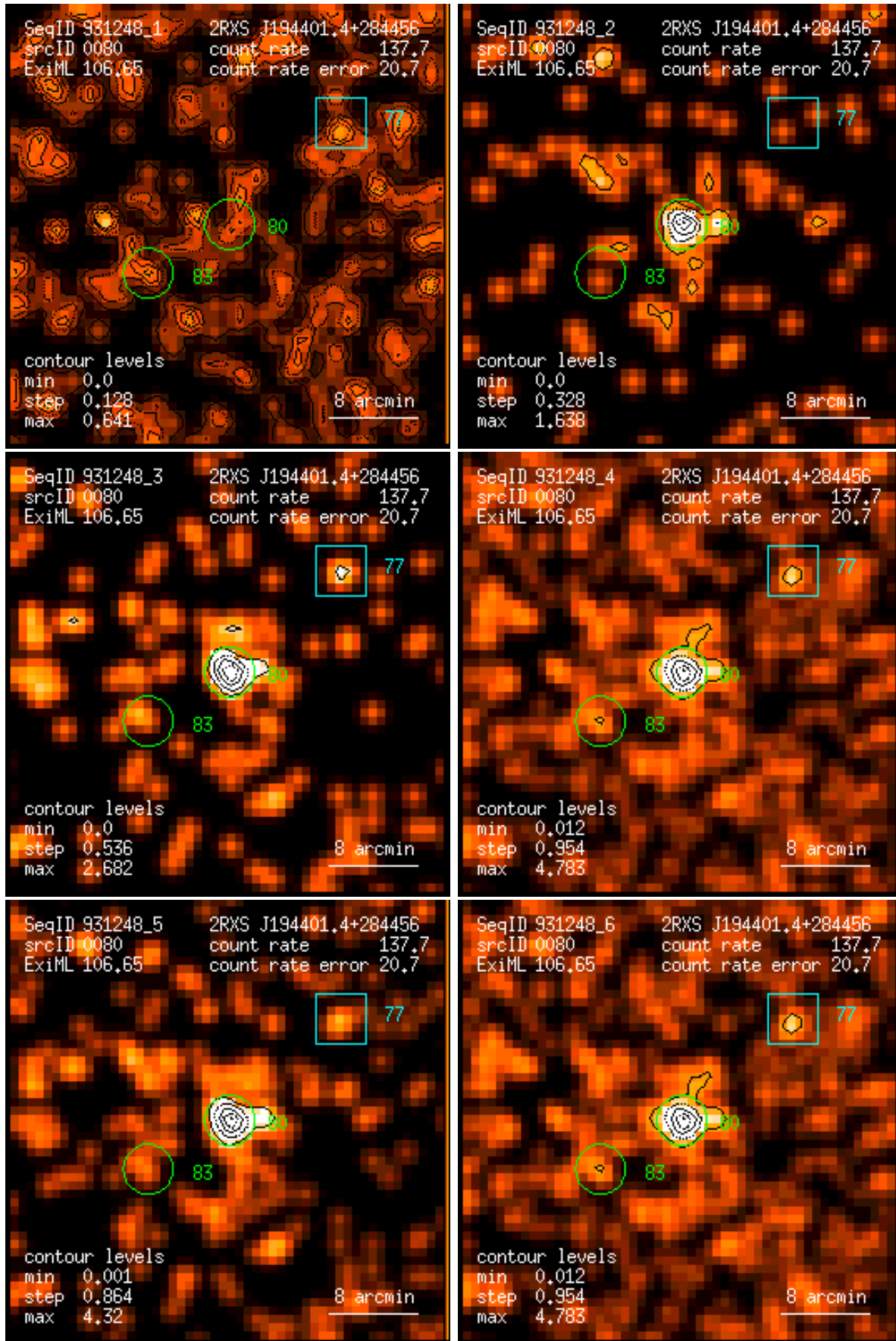
Figure 80: RASS 931248: detection 0080: band rate images, Gaussian filter: (1) PSPC channels 11 – 41, (2) 52 – 90, (3) 91 – 201, (4) 11 – 235, (5) 52 – 201, (6) 11 – 201. Broad band rates in counts/ks. Band rate contour levels in counts/ks/arcmin 2 .
