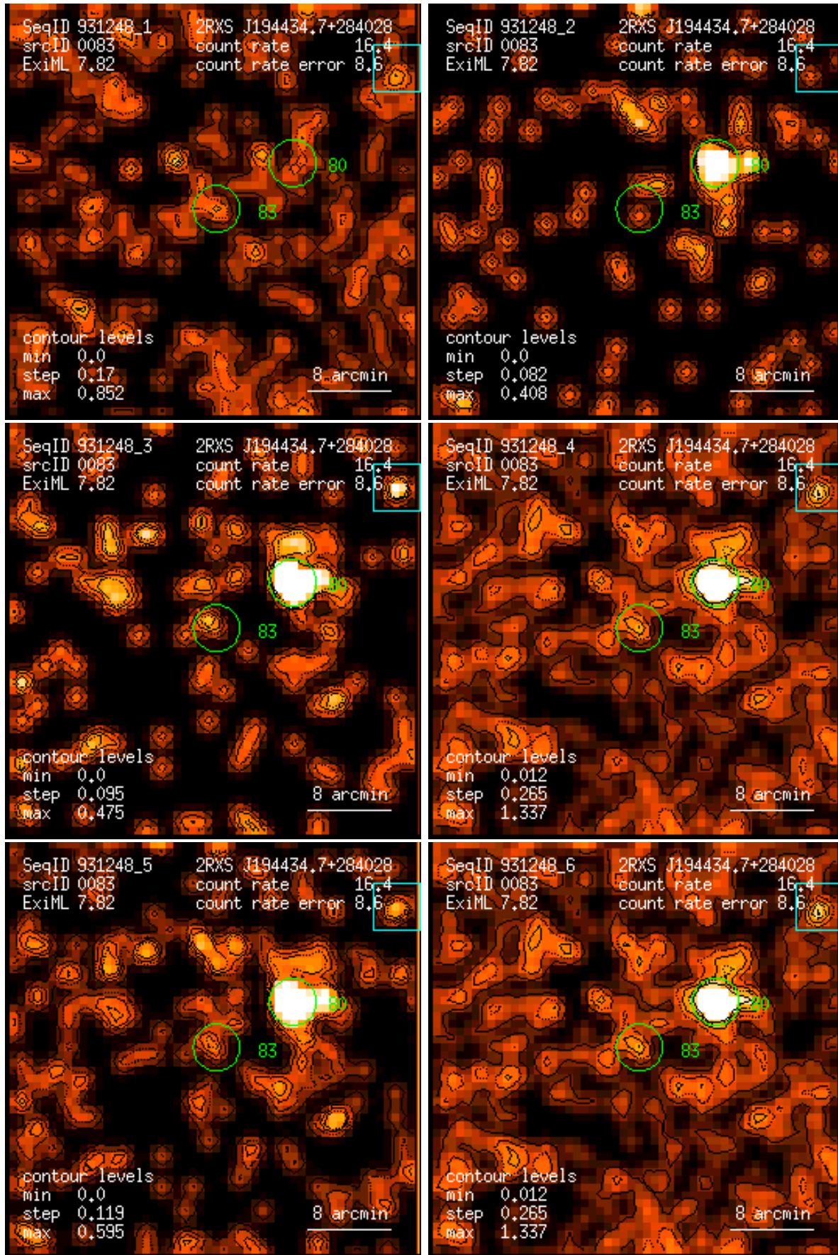
Figure 83: RASS 931248: detection 0083: band rate images, Gaussian filter: (1) PSPC channels 11 – 41, (2) 52 – 90, (3) 91 – 201, (4) 11 – 235, (5) 52 – 201, (6) 11 – 201. Broad band rates in counts/ks. Band rate contour levels in counts/ks/arcmin 2 .
