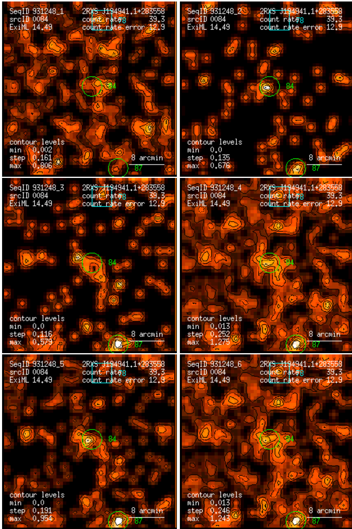
Figure 84: RASS 931248: detection 0084: band rate images, Gaussian filter: (1) PSPC channels 11 – 41, (2) 52 – 90, (3) 91 – 201, (4) 11 – 235, (5) 52 – 201, (6) 11 – 201. Broad band rates in counts/ks. Band rate contour levels in counts/ks/arcmin 2 .
