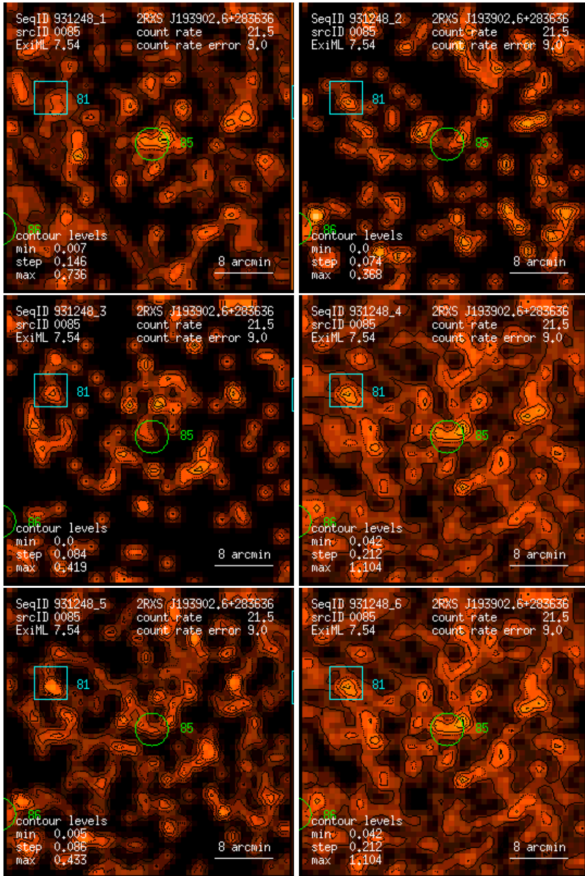
Figure 85: RASS 931248: detection 0085: band rate images, Gaussian filter: (1) PSPC channels 11 – 41, (2) 52 – 90, (3) 91 – 201, (4) 11 – 235, (5) 52 – 201, (6) 11 – 201. Broad band rates in counts/ks. Band rate contour levels in counts/ks/arcmin 2 .
