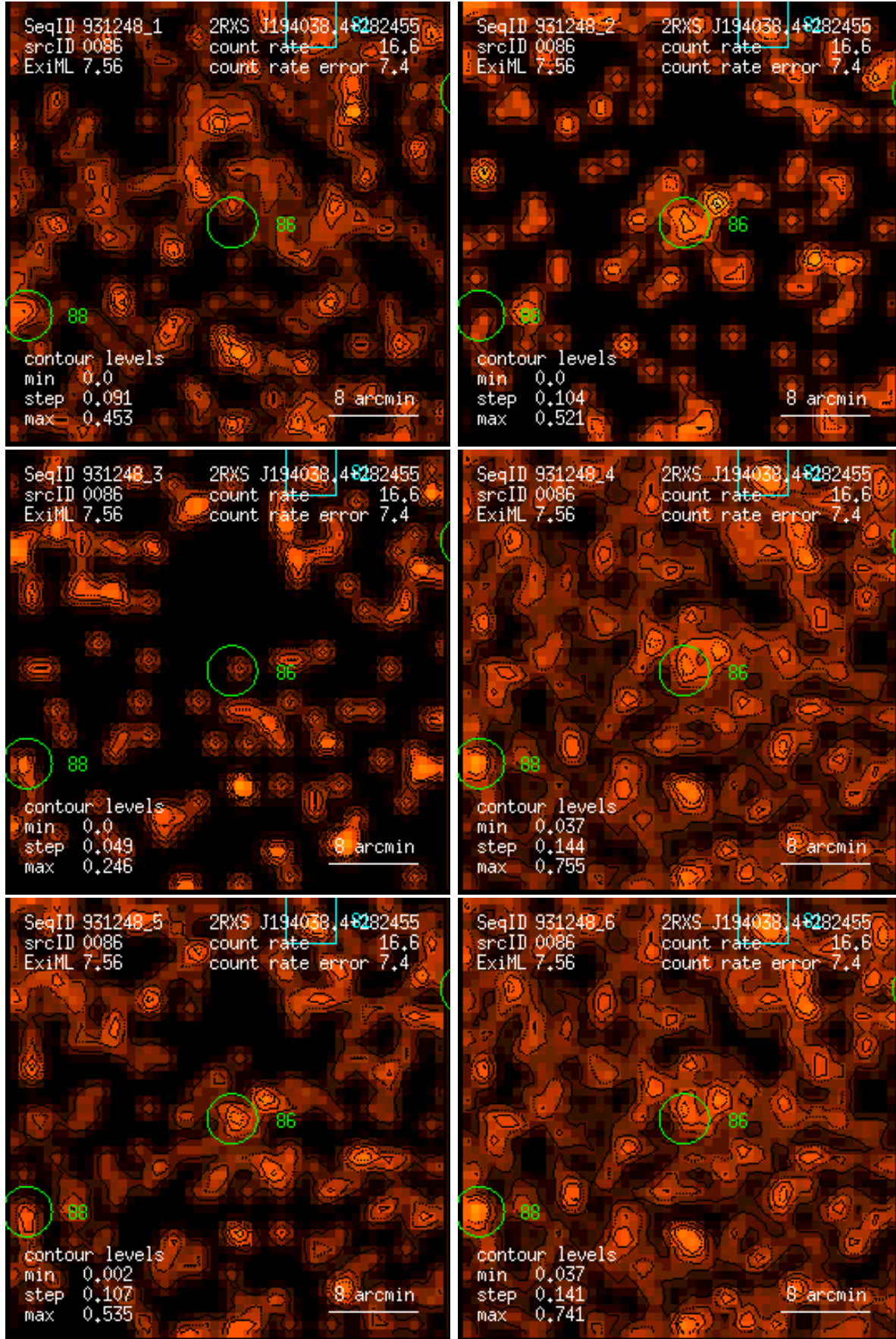
Figure 86: RASS 931248: detection 0086: band rate images, Gaussian filter: (1) PSPC channels 11 – 41, (2) 52 – 90, (3) 91 – 201, (4) 11 – 235, (5) 52 – 201, (6) 11 – 201. Broad band rates in counts/ks. Band rate contour levels in counts/ks/arcmin 2 .
