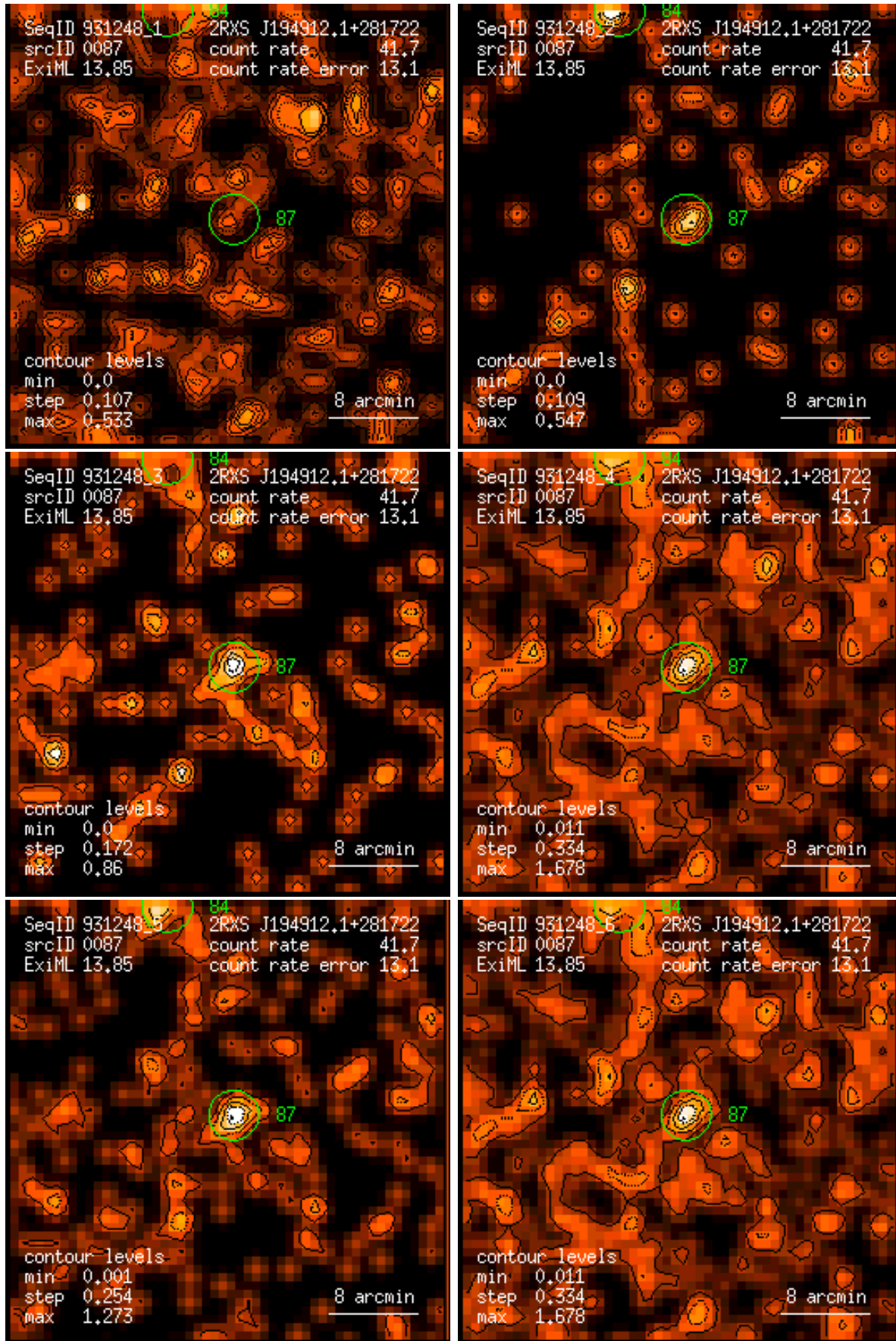
Figure 87: RASS 931248: detection 0087: band rate images, Gaussian filter: (1) PSPC channels 11 – 41, (2) 52 – 90, (3) 91 – 201, (4) 11 – 235, (5) 52 – 201, (6) 11 – 201. Broad band rates in counts/ks. Band rate contour levels in counts/ks/arcmin 2 .
