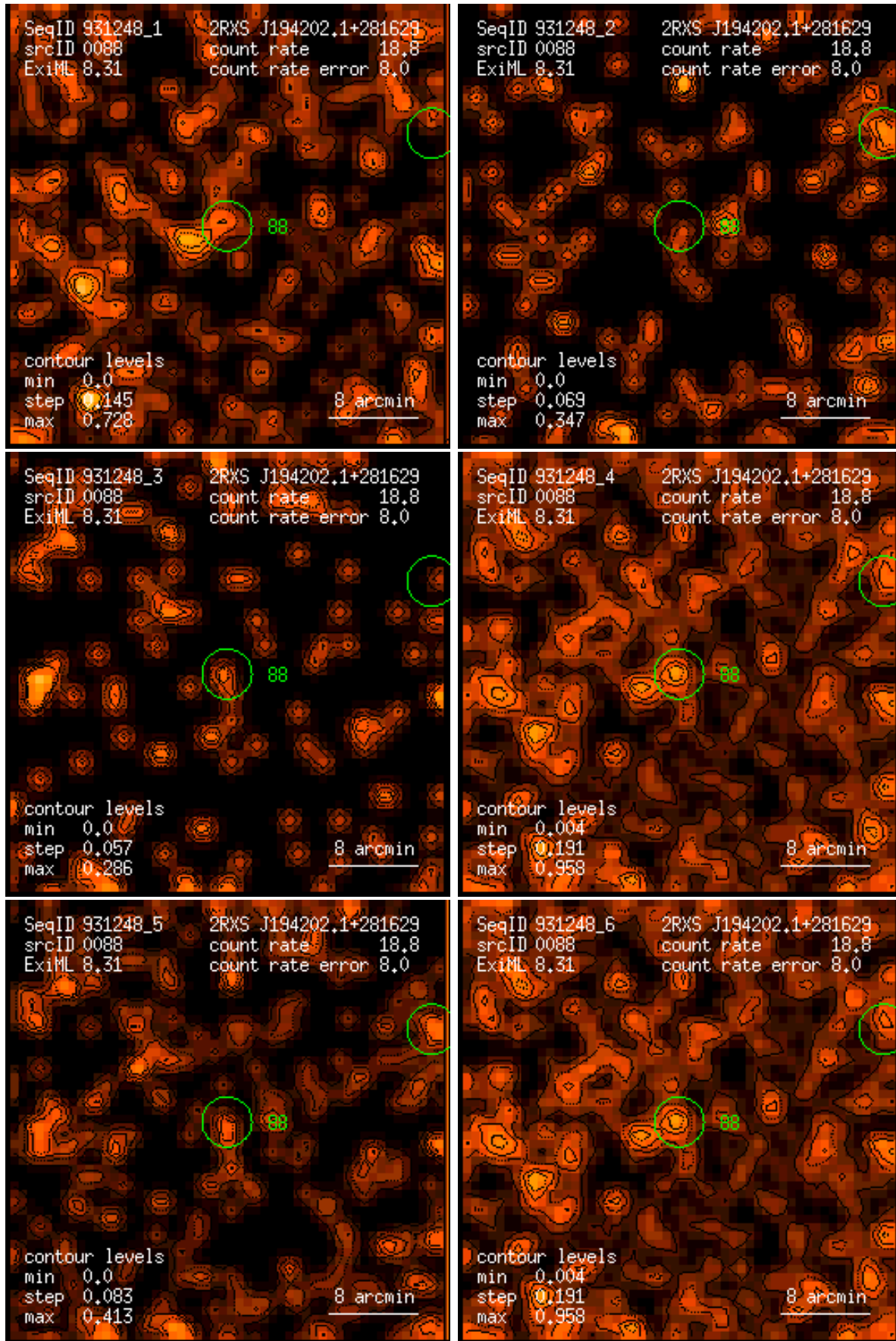
Figure 88: RASS 931248: detection 0088: band rate images, Gaussian filter: (1) PSPC channels 11 – 41, (2) 52 – 90, (3) 91 – 201, (4) 11 – 235, (5) 52 – 201, (6) 11 – 201. Broad band rates in counts/ks. Band rate contour levels in counts/ks/arcmin 2 .
