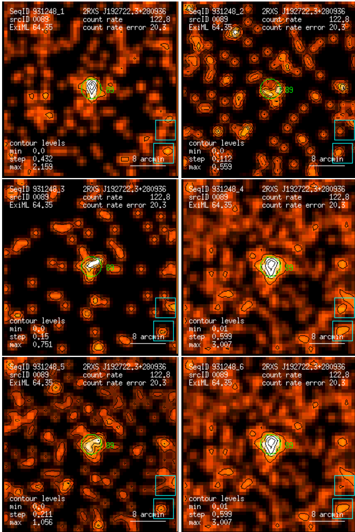
Figure 89: RASS 931248: detection 0089: band rate images, Gaussian filter: (1) PSPC channels 11 – 41, (2) 52 – 90, (3) 91 – 201, (4) 11 – 235, (5) 52 – 201, (6) 11 – 201. Broad band rates in counts/ks. Band rate contour levels in counts/ks/arcmin 2 .
