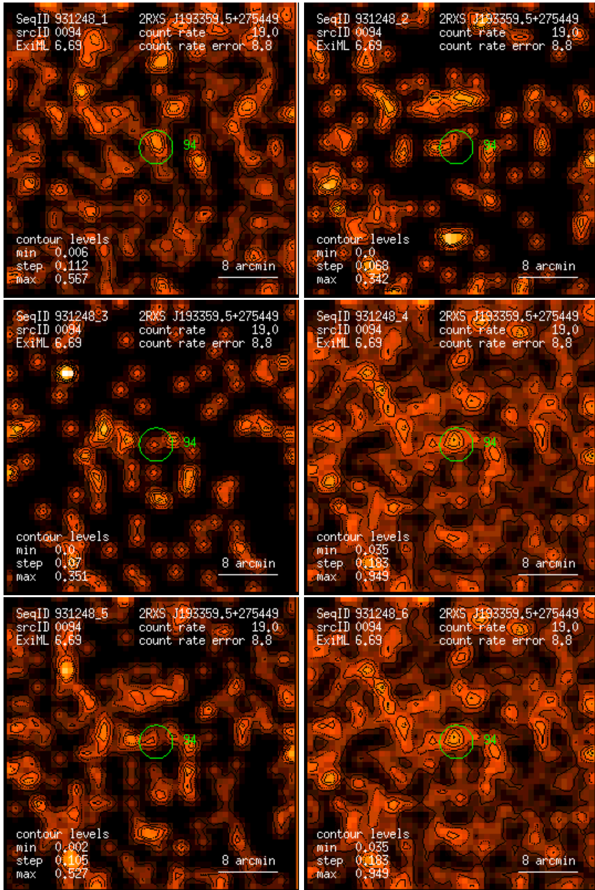
Figure 94: RASS 931248: detection 0094: band rate images, Gaussian filter: (1) PSPC channels 11 – 41, (2) 52 – 90, (3) 91 – 201, (4) 11 – 235, (5) 52 – 201, (6) 11 – 201. Broad band rates in counts/ks. Band rate contour levels in counts/ks/arcmin 2 .
