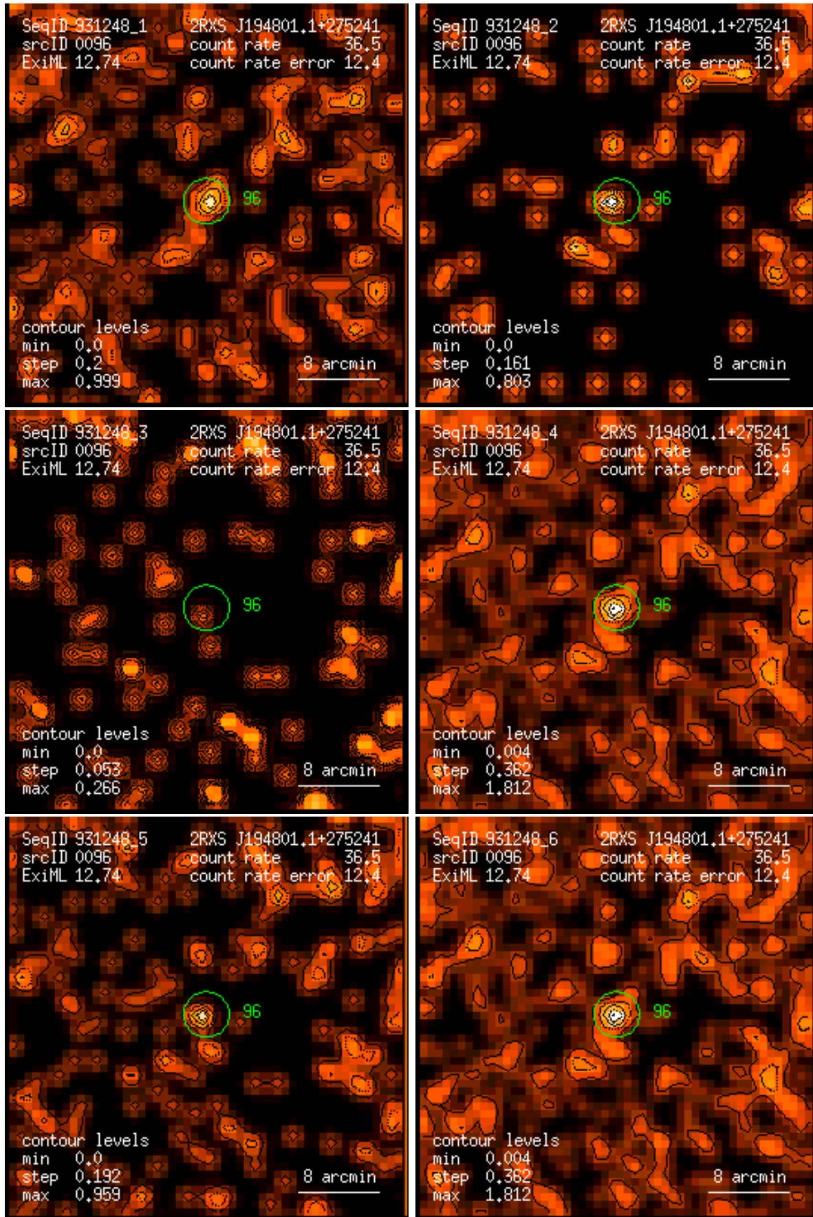
Figure 96: RASS 931248: detection 0096: band rate images, Gaussian filter: (1) PSPC channels 11 – 41, (2) 52 – 90, (3) 91 – 201, (4) 11 – 235, (5) 52 – 201, (6) 11 – 201. Broad band rates in counts/ks. Band rate contour levels in counts/ks/arcmin 2 .
