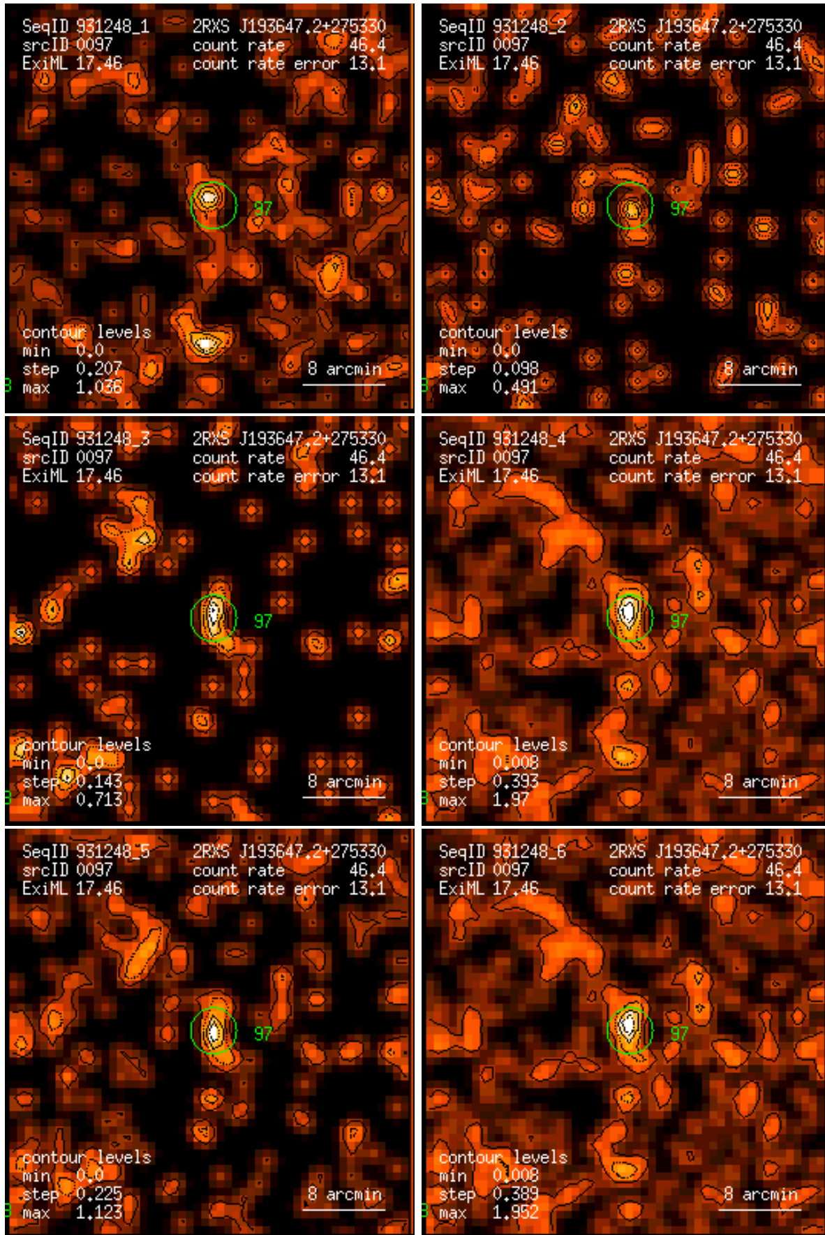
Figure 97: RASS 931248: detection 0097: band rate images, Gaussian filter: (1) PSPC channels 11 – 41, (2) 52 – 90, (3) 91 – 201, (4) 11 – 235, (5) 52 – 201, (6) 11 – 201. Broad band rates in counts/ks. Band rate contour levels in counts/ks/arcmin 2 .
