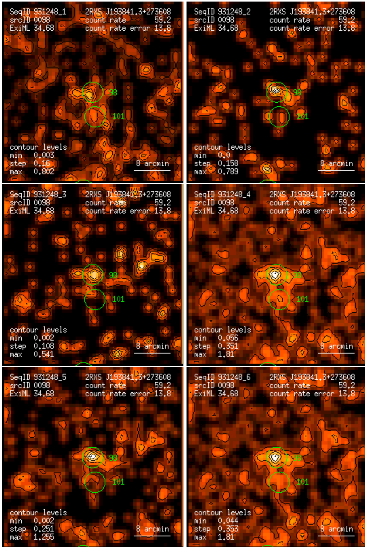
Figure 98: RASS 931248: detection 0098: band rate images, Gaussian filter: (1) PSPC channels 11 – 41, (2) 52 – 90, (3) 91 – 201, (4) 11 – 235, (5) 52 – 201, (6) 11 – 201. Broad band rates in counts/ks. Band rate contour levels in counts/ks/arcmin 2 .
