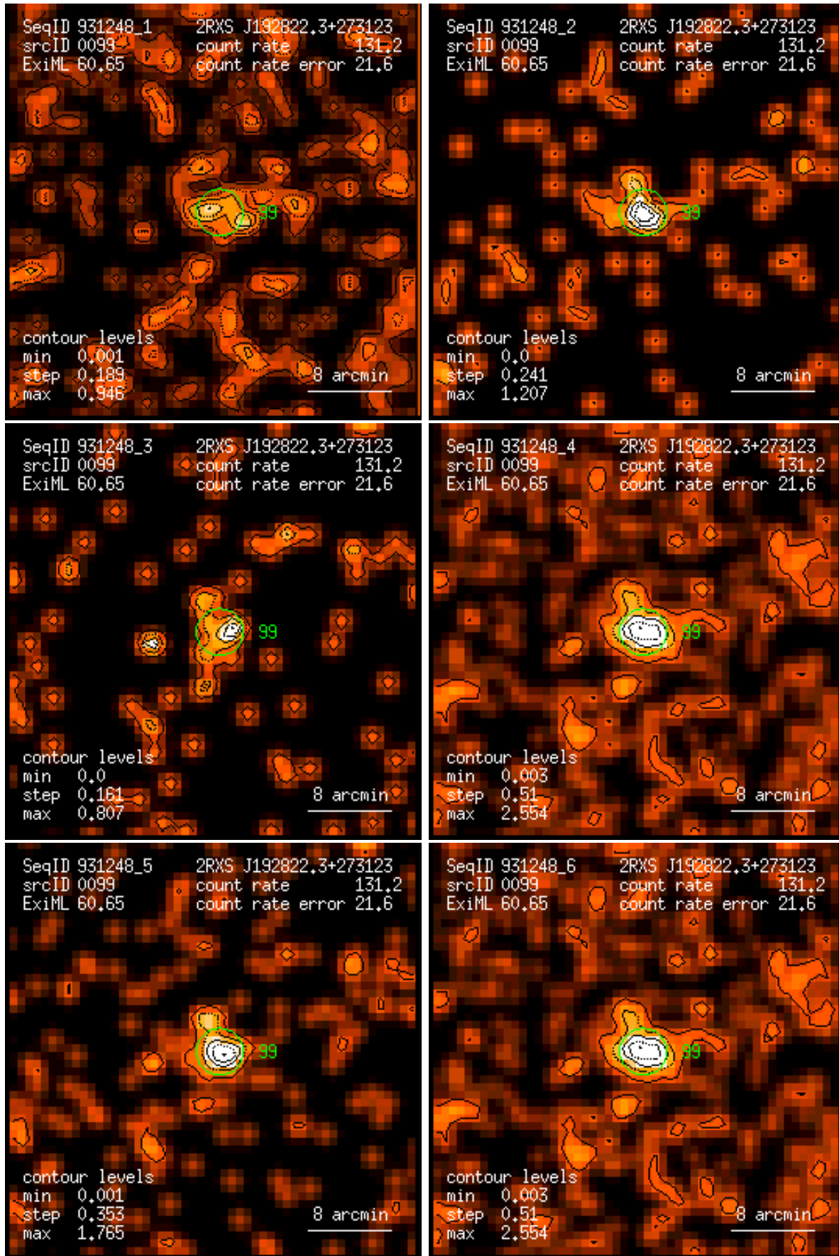
Figure 99: RASS 931248: detection 0099: band rate images, Gaussian filter: (1) PSPC channels 11 – 41, (2) 52 – 90, (3) 91 – 201, (4) 11 – 235, (5) 52 – 201, (6) 11 – 201. Broad band rates in counts/ks. Band rate contour levels in counts/ks/arcmin 2 .
