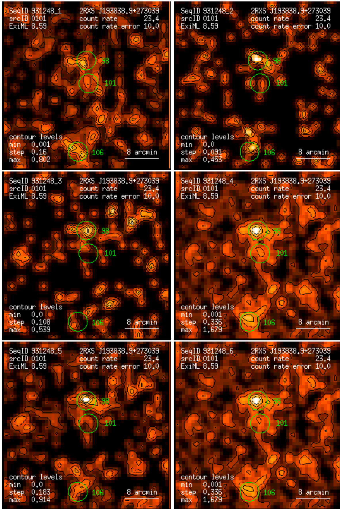
Figure 101: RASS 931248: detection 0101: band rate images, Gaussian filter: (1) PSPC channels 11 – 41, (2) 52 – 90, (3) 91 – 201, (4) 11 – 235, (5) 52 – 201, (6) 11 – 201. Broad band rates in counts/ks. Band rate contour levels in counts/ks/arcmin 2 .
