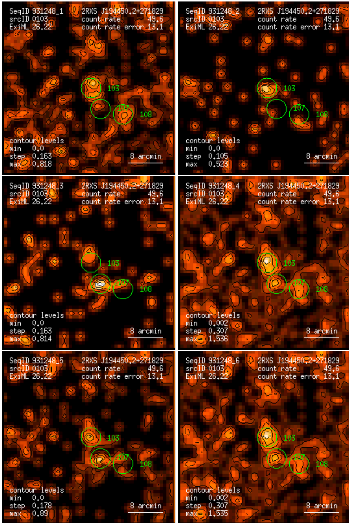
Figure 103: RASS 931248: detection 0103: band rate images, Gaussian filter: (1) PSPC channels 11 – 41, (2) 52 – 90, (3) 91 – 201, (4) 11 – 235, (5) 52 – 201, (6) 11 – 201. Broad band rates in counts/ks. Band rate contour levels in counts/ks/arcmin 2 .
