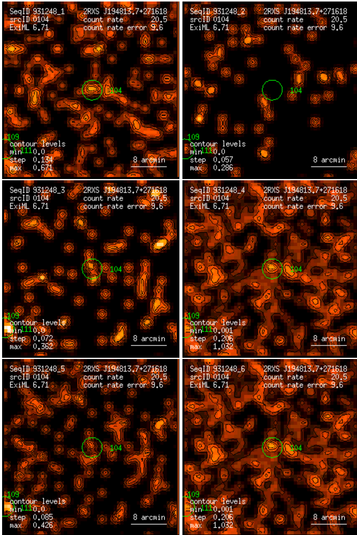
Figure 104: RASS 931248: detection 0104: band rate images, Gaussian filter: (1) PSPC channels 11 – 41, (2) 52 – 90, (3) 91 – 201, (4) 11 – 235, (5) 52 – 201, (6) 11 – 201. Broad band rates in counts/ks. Band rate contour levels in counts/ks/arcmin 2 .
