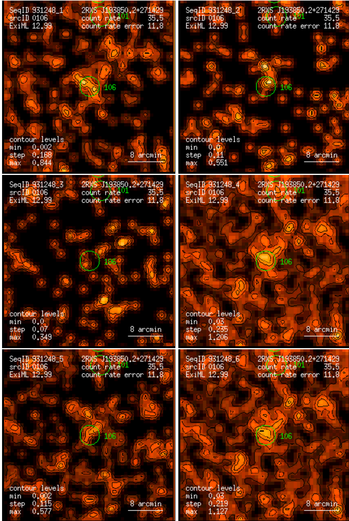
Figure 106: RASS 931248: detection 0106: band rate images, Gaussian filter: (1) PSPC channels 11 – 41, (2) 52 – 90, (3) 91 – 201, (4) 11 – 235, (5) 52 – 201, (6) 11 – 201. Broad band rates in counts/ks. Band rate contour levels in counts/ks/arcmin 2 .
