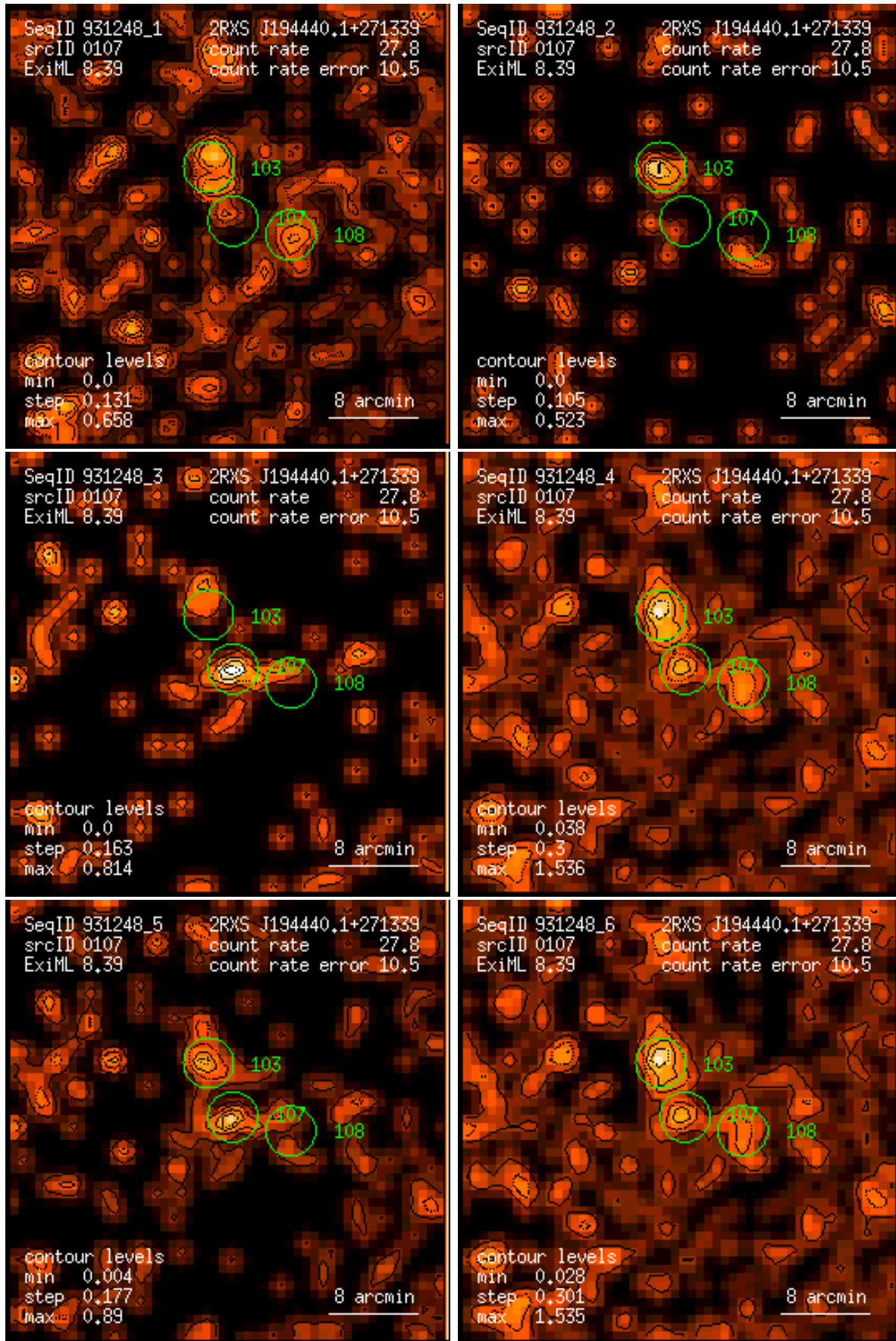
Figure 107: RASS 931248: detection 0107: band rate images, Gaussian filter: (1) PSPC channels 11 – 41, (2) 52 – 90, (3) 91 – 201, (4) 11 – 235, (5) 52 – 201, (6) 11 – 201. Broad band rates in counts/ks. Band rate contour levels in counts/ks/arcmin 2 .
