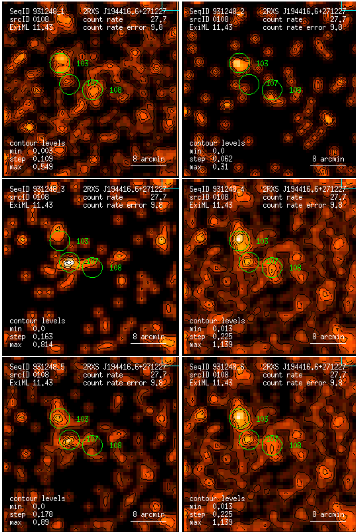
Figure 108: RASS 931248: detection 0108: band rate images, Gaussian filter: (1) PSPC channels 11 – 41, (2) 52 – 90, (3) 91 – 201, (4) 11 – 235, (5) 52 – 201, (6) 11 – 201. Broad band rates in counts/ks. Band rate contour levels in counts/ks/arcmin 2 .
