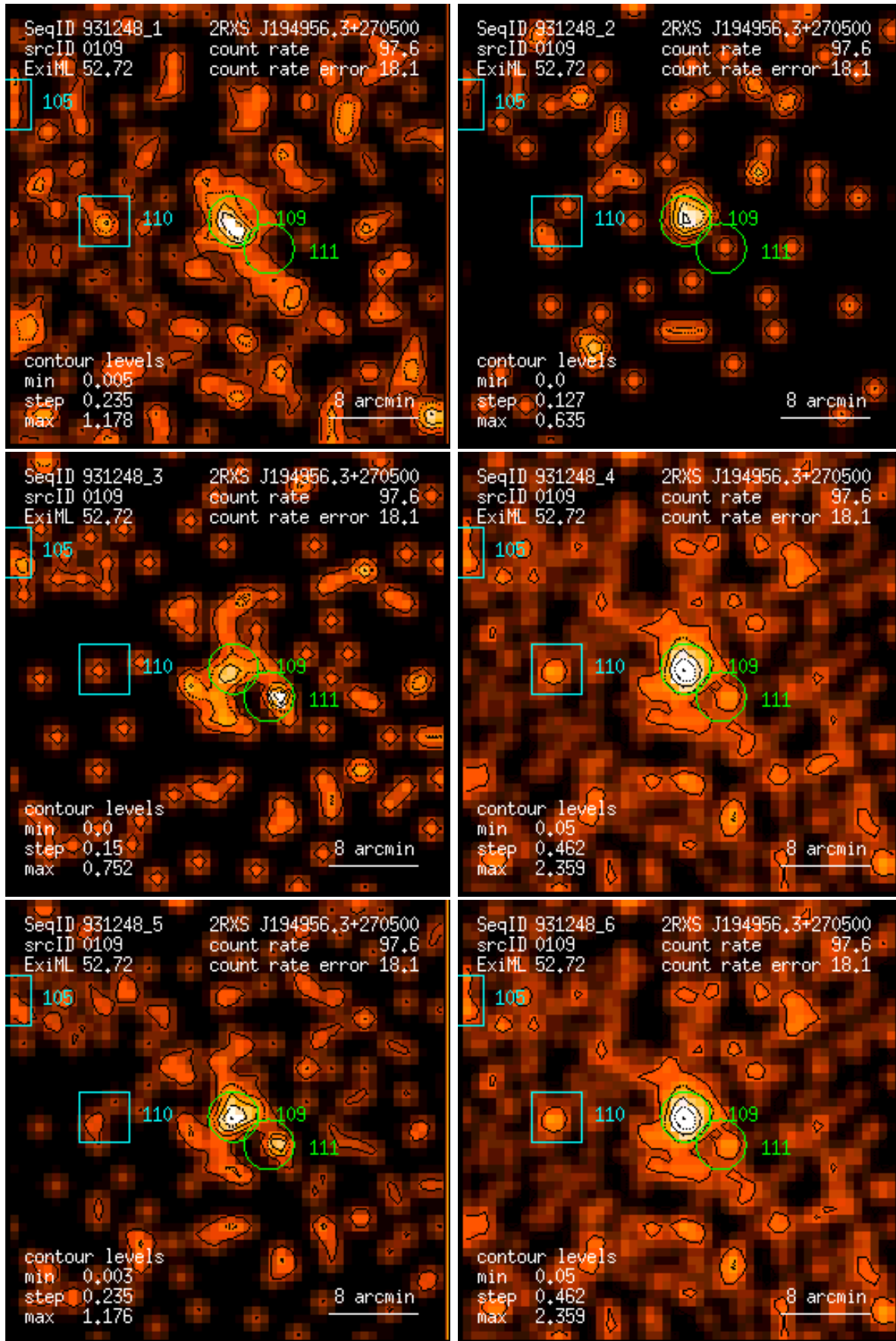
Figure 109: RASS 931248: detection 0109: band rate images, Gaussian filter: (1) PSPC channels 11 – 41, (2) 52 – 90, (3) 91 – 201, (4) 11 – 235, (5) 52 – 201, (6) 11 – 201. Broad band rates in counts/ks. Band rate contour levels in counts/ks/arcmin 2 .
