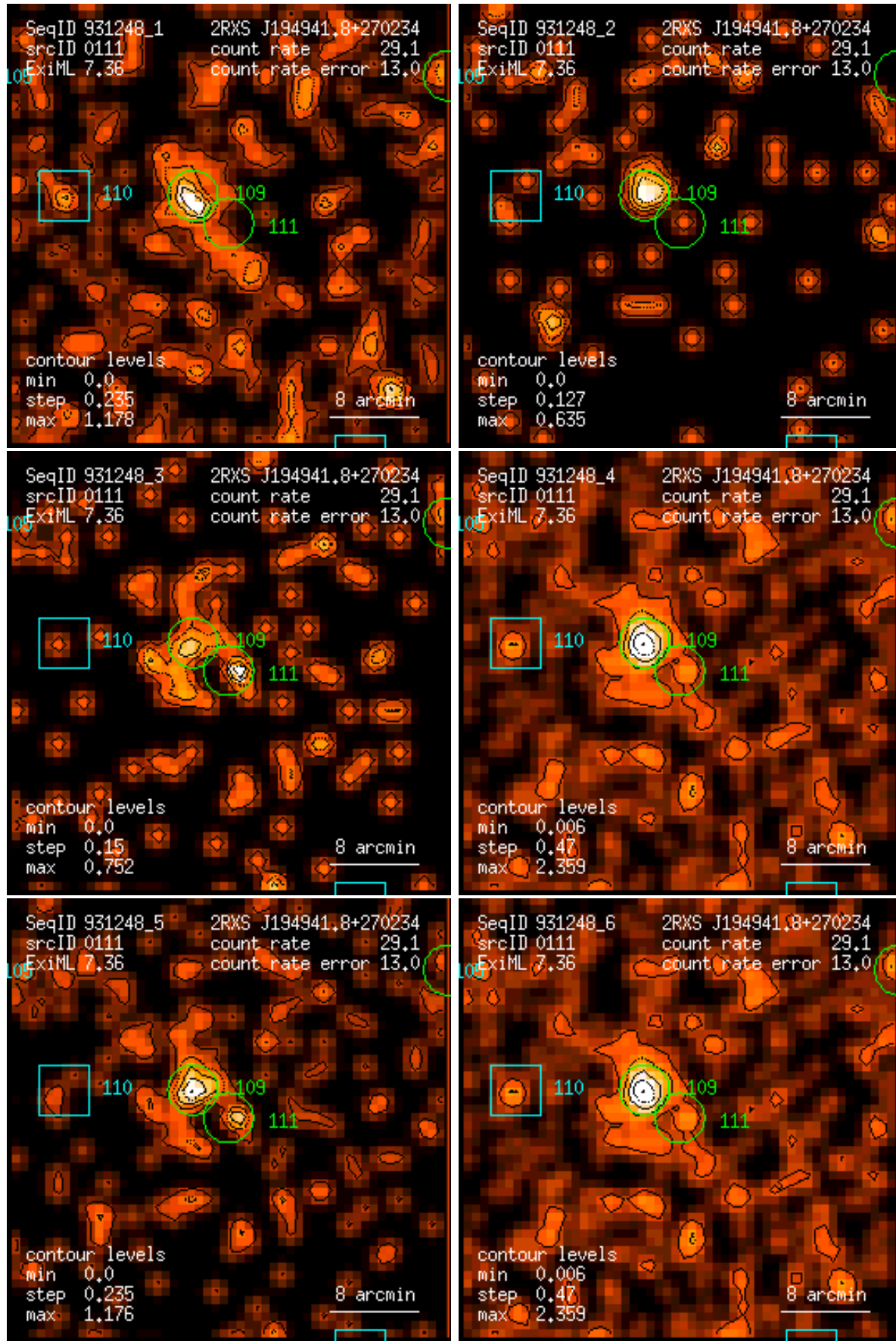
Figure 111: RASS 931248: detection 0111: band rate images, Gaussian filter: (1) PSPC channels 11 – 41, (2) 52 – 90, (3) 91 – 201, (4) 11 – 235, (5) 52 – 201, (6) 11 – 201. Broad band rates in counts/ks. Band rate contour levels in counts/ks/arcmin 2 .
