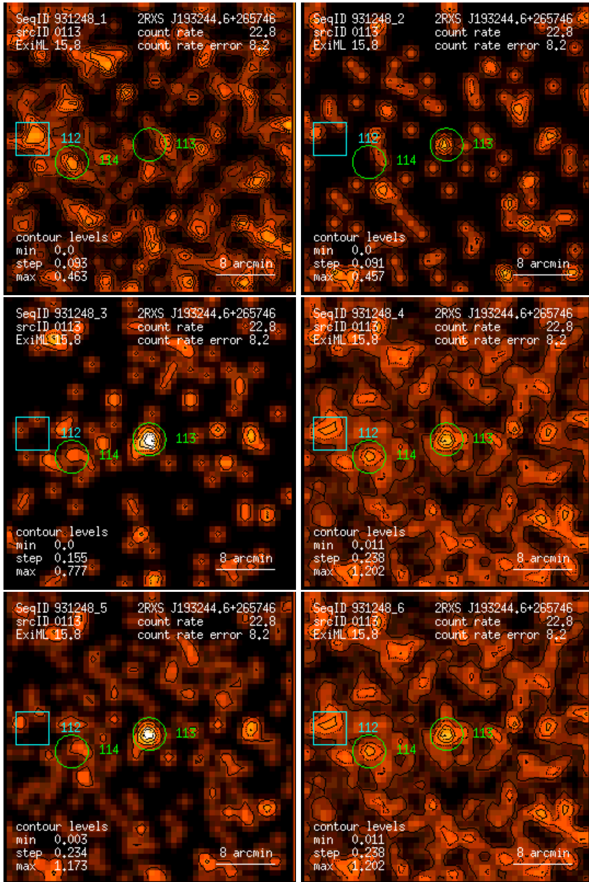
Figure 113: RASS 931248: detection 0113: band rate images, Gaussian filter: (1) PSPC channels 11 – 41, (2) 52 – 90, (3) 91 – 201, (4) 11 – 235, (5) 52 – 201, (6) 11 – 201. Broad band rates in counts/ks. Band rate contour levels in counts/ks/arcmin 2 .
