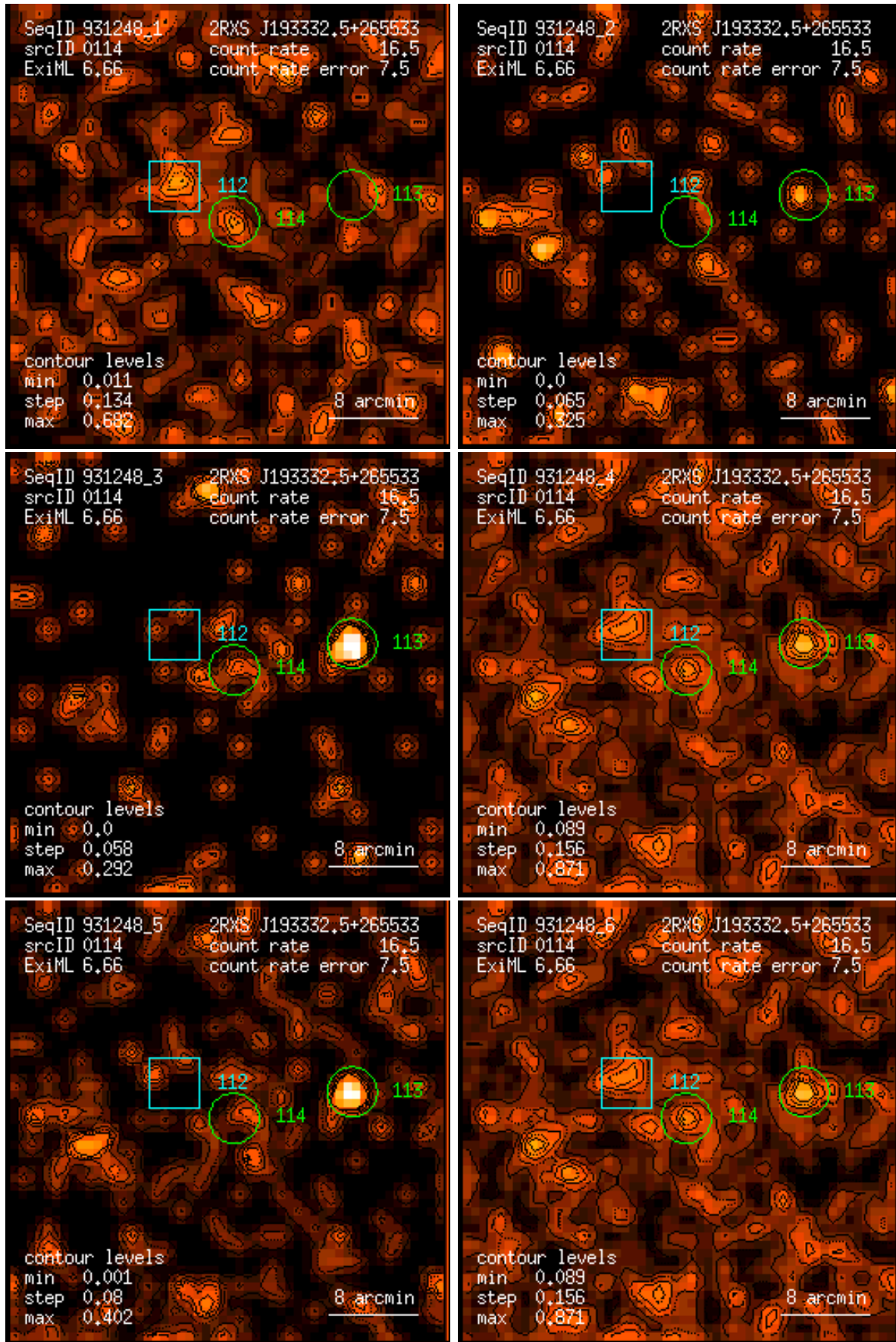
Figure 114: RASS 931248: detection 0114: band rate images, Gaussian filter: (1) PSPC channels 11 – 41, (2) 52 – 90, (3) 91 – 201, (4) 11 – 235, (5) 52 – 201, (6) 11 – 201. Broad band rates in counts/ks. Band rate contour levels in counts/ks/arcmin 2 .
